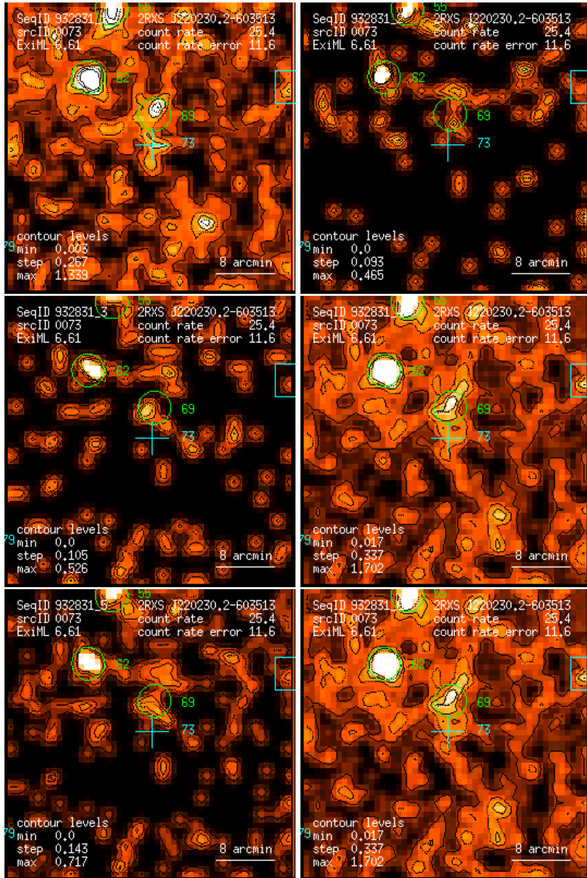
Figure 73: RASS 932831: detection 0073: band rate images, Gaussian filter: (1) PSPC channels 11 – 41, (2) 52 – 90, (3) 91 – 201, (4) 11 – 235, (5) 52 – 201, (6) 11 – 201. Broad band rates in counts/ks. Band rate contour levels in counts/ks/arcmin 2 .
