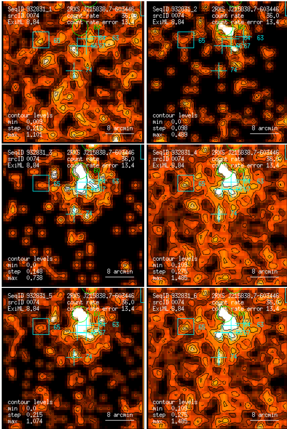
Figure 74: RASS 932831: detection 0074: band rate images, Gaussian filter: (1) PSPC channels 11 – 41, (2) 52 – 90, (3) 91 – 201, (4) 11 – 235, (5) 52 – 201, (6) 11 – 201. Broad band rates in counts/ks. Band rate contour levels in counts/ks/arcmin 2 .
