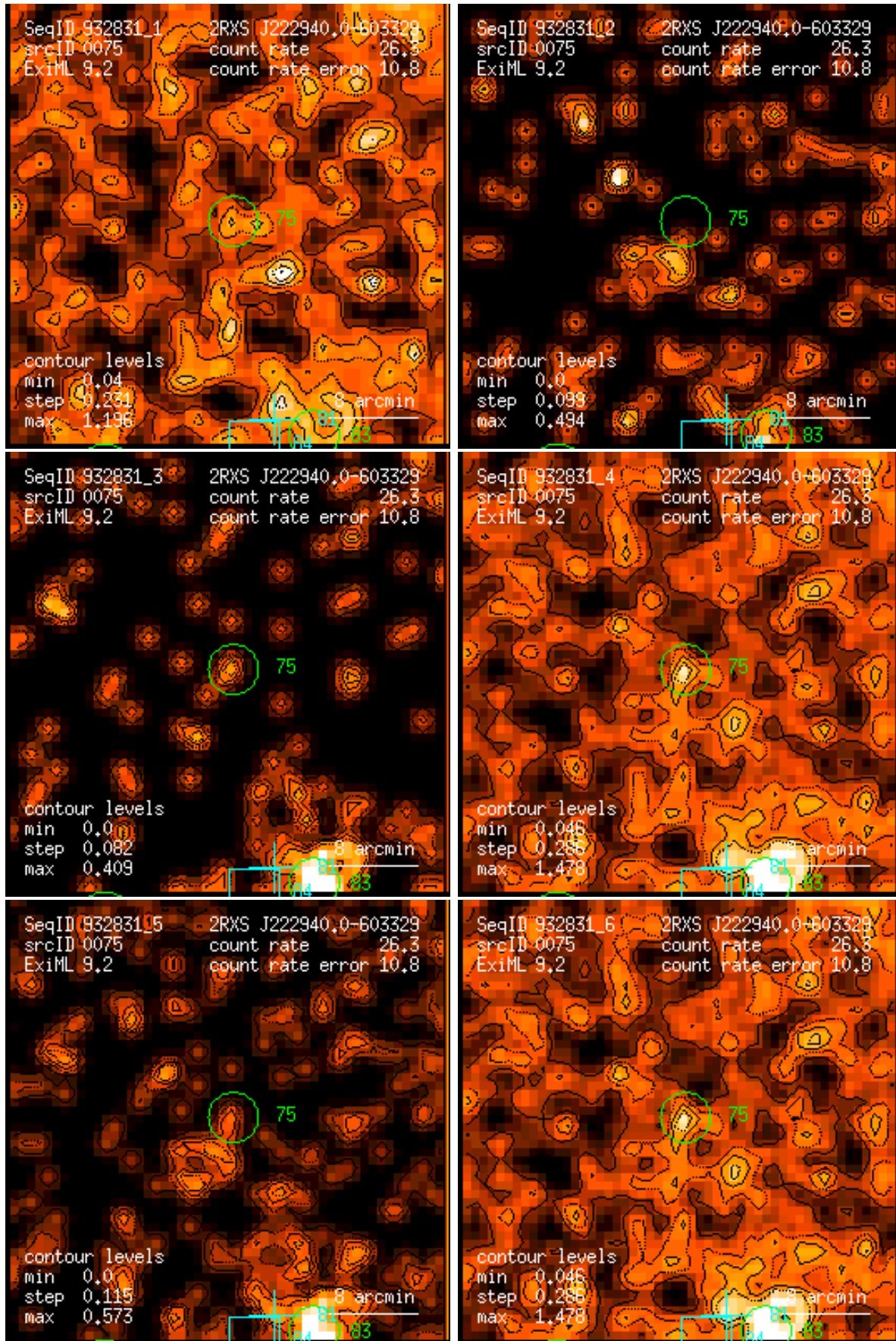
Figure 75: RASS 932831: detection 0075: band rate images, Gaussian filter: (1) PSPC channels 11 – 41, (2) 52 – 90, (3) 91 – 201, (4) 11 – 235, (5) 52 – 201, (6) 11 – 201. Broad band rates in counts/ks. Band rate contour levels in counts/ks/arcmin 2 .
