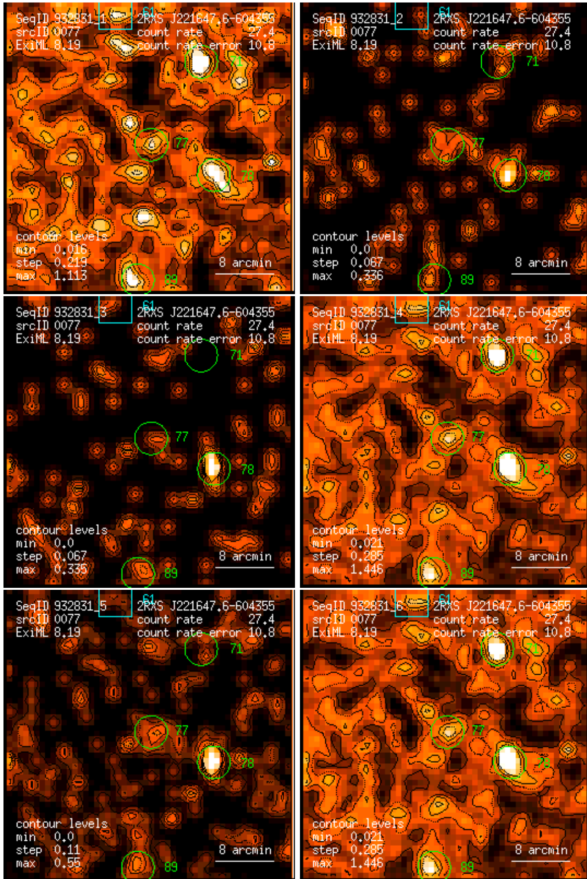
Figure 77: RASS 932831: detection 0077: band rate images, Gaussian filter: (1) PSPC channels 11 – 41, (2) 52 – 90, (3) 91 – 201, (4) 11 – 235, (5) 52 – 201, (6) 11 – 201. Broad band rates in counts/ks. Band rate contour levels in counts/ks/arcmin 2 .
