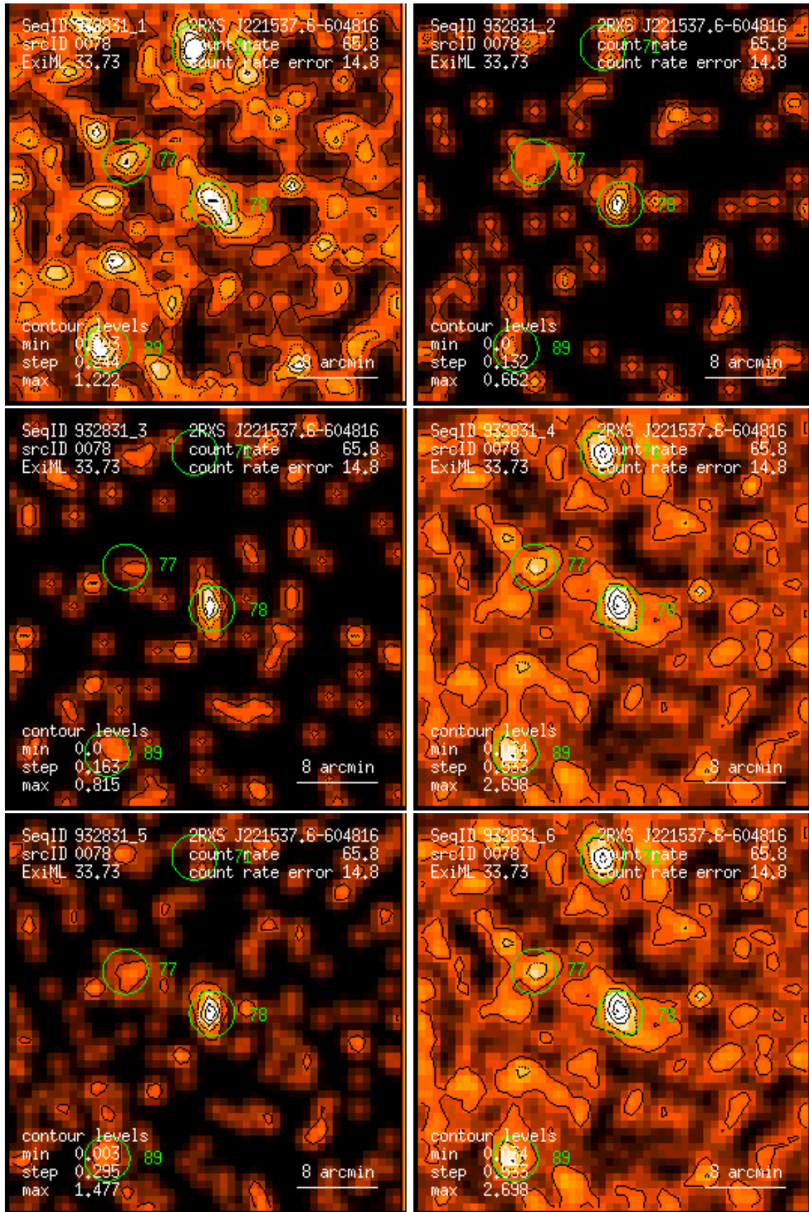
Figure 78: RASS 932831: detection 0078: band rate images, Gaussian filter: (1) PSPC channels 11 – 41, (2) 52 – 90, (3) 91 – 201, (4) 11 – 235, (5) 52 – 201, (6) 11 – 201. Broad band rates in counts/ks. Band rate contour levels in counts/ks/arcmin 2 .
