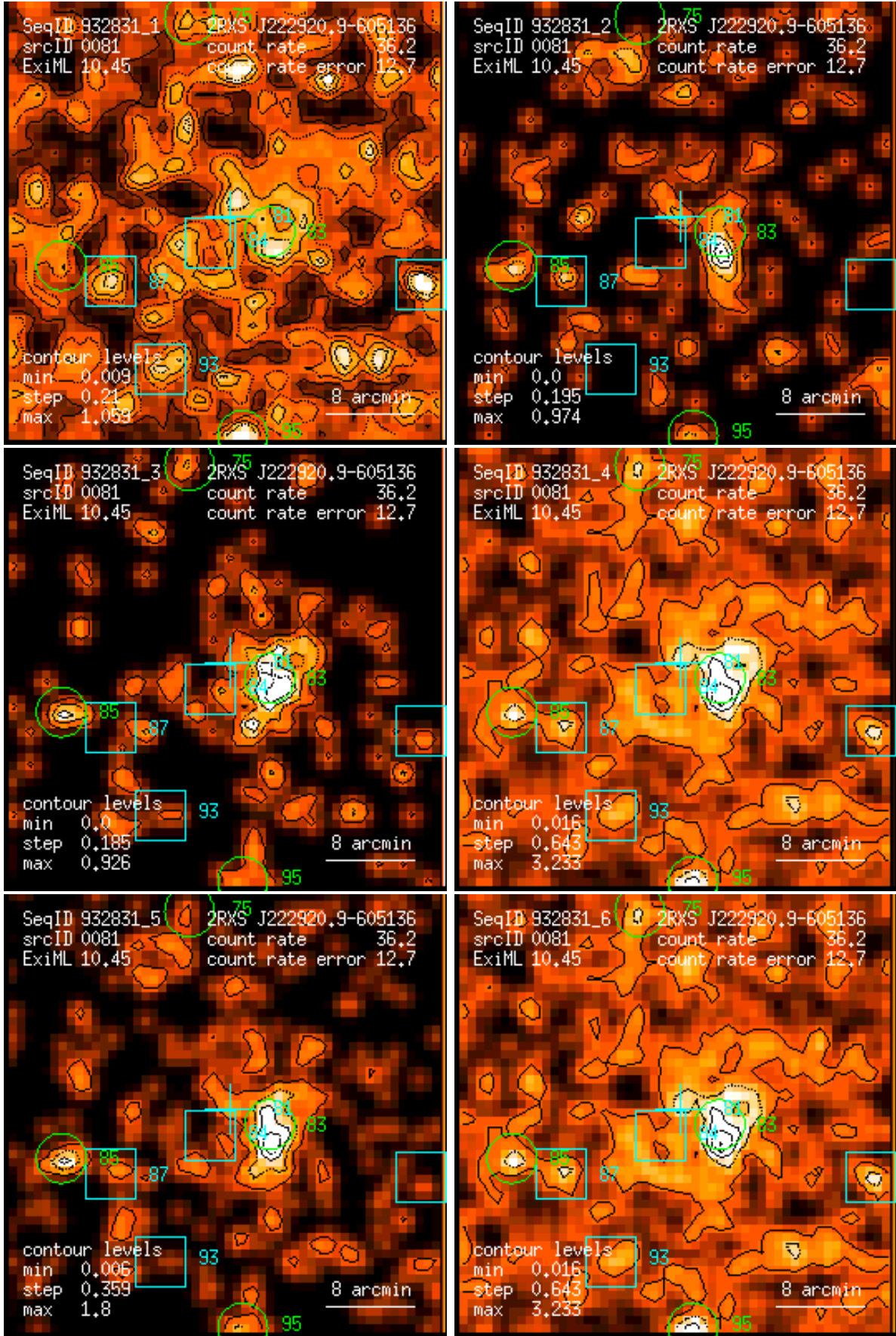
Figure 81: RASS 932831: detection 0081: band rate images, Gaussian filter: (1) PSPC channels 11 – 41, (2) 52 – 90, (3) 91 – 201, (4) 11 – 235, (5) 52 – 201, (6) 11 – 201. Broad band rates in counts/ks. Band rate contour levels in counts/ks/arcmin 2 .
