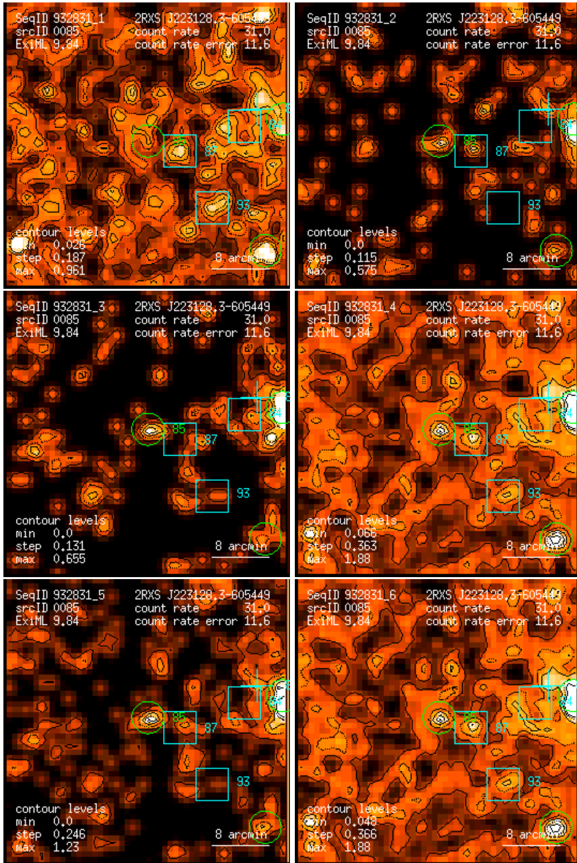
Figure 85: RASS 932831: detection 0085: band rate images, Gaussian filter: (1) PSPC channels 11 – 41, (2) 52 – 90, (3) 91 – 201, (4) 11 – 235, (5) 52 – 201, (6) 11 – 201. Broad band rates in counts/ks. Band rate contour levels in counts/ks/arcmin 2 .
