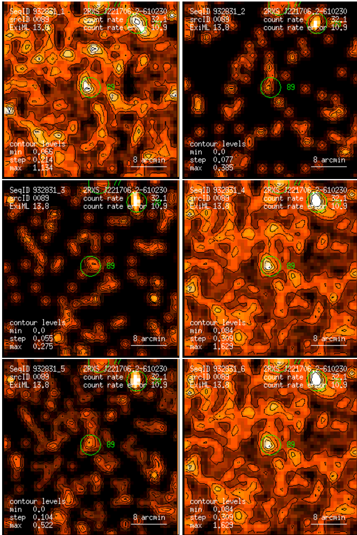
Figure 89: RASS 932831: detection 0089: band rate images, Gaussian filter: (1) PSPC channels 11 – 41, (2) 52 – 90, (3) 91 – 201, (4) 11 – 235, (5) 52 – 201, (6) 11 – 201. Broad band rates in counts/ks. Band rate contour levels in counts/ks/arcmin 2 .
