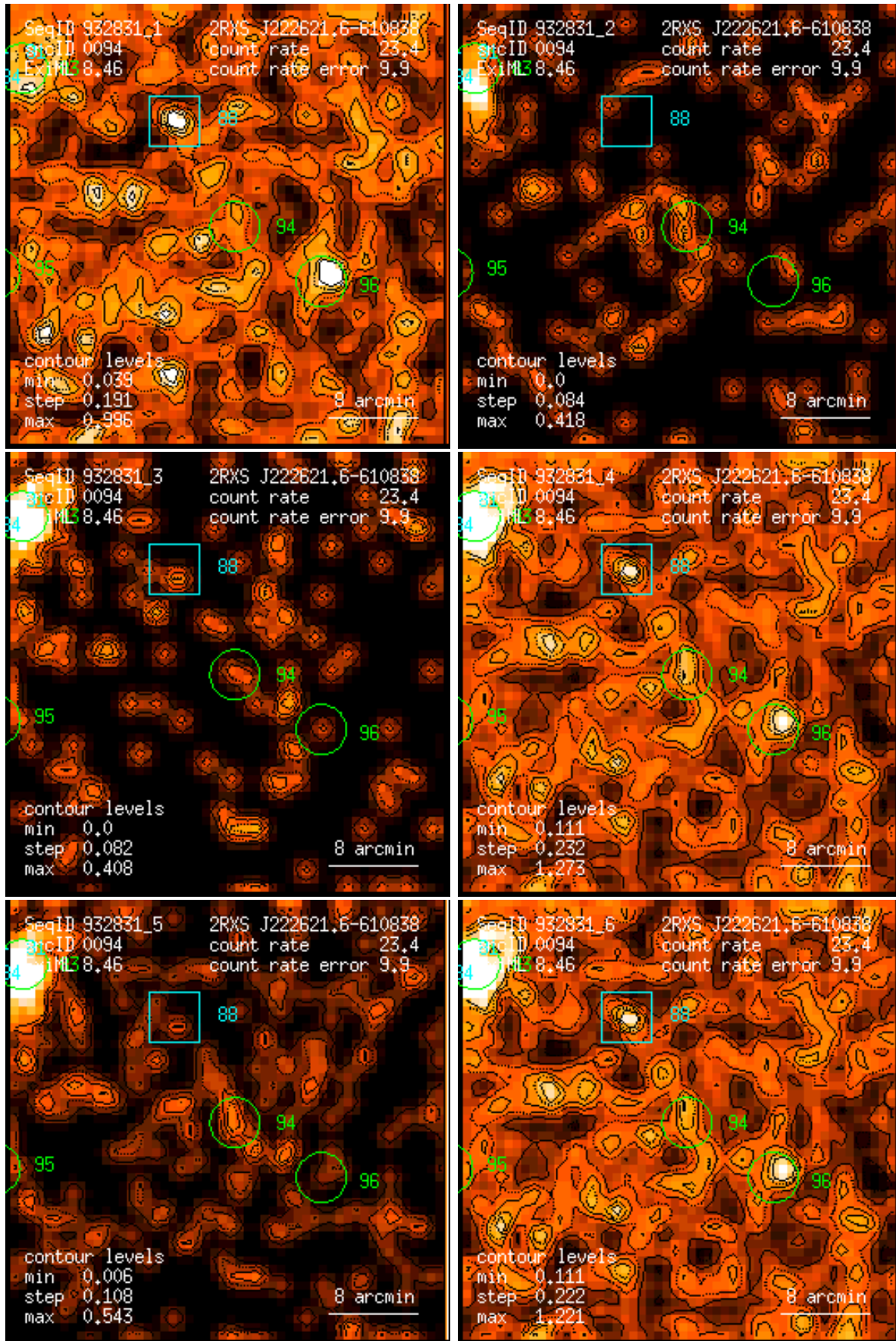
Figure 94: RASS 932831: detection 0094: band rate images, Gaussian filter: (1) PSPC channels 11 – 41, (2) 52 – 90, (3) 91 – 201, (4) 11 – 235, (5) 52 – 201, (6) 11 – 201. Broad band rates in counts/ks. Band rate contour levels in counts/ks/arcmin 2 .
