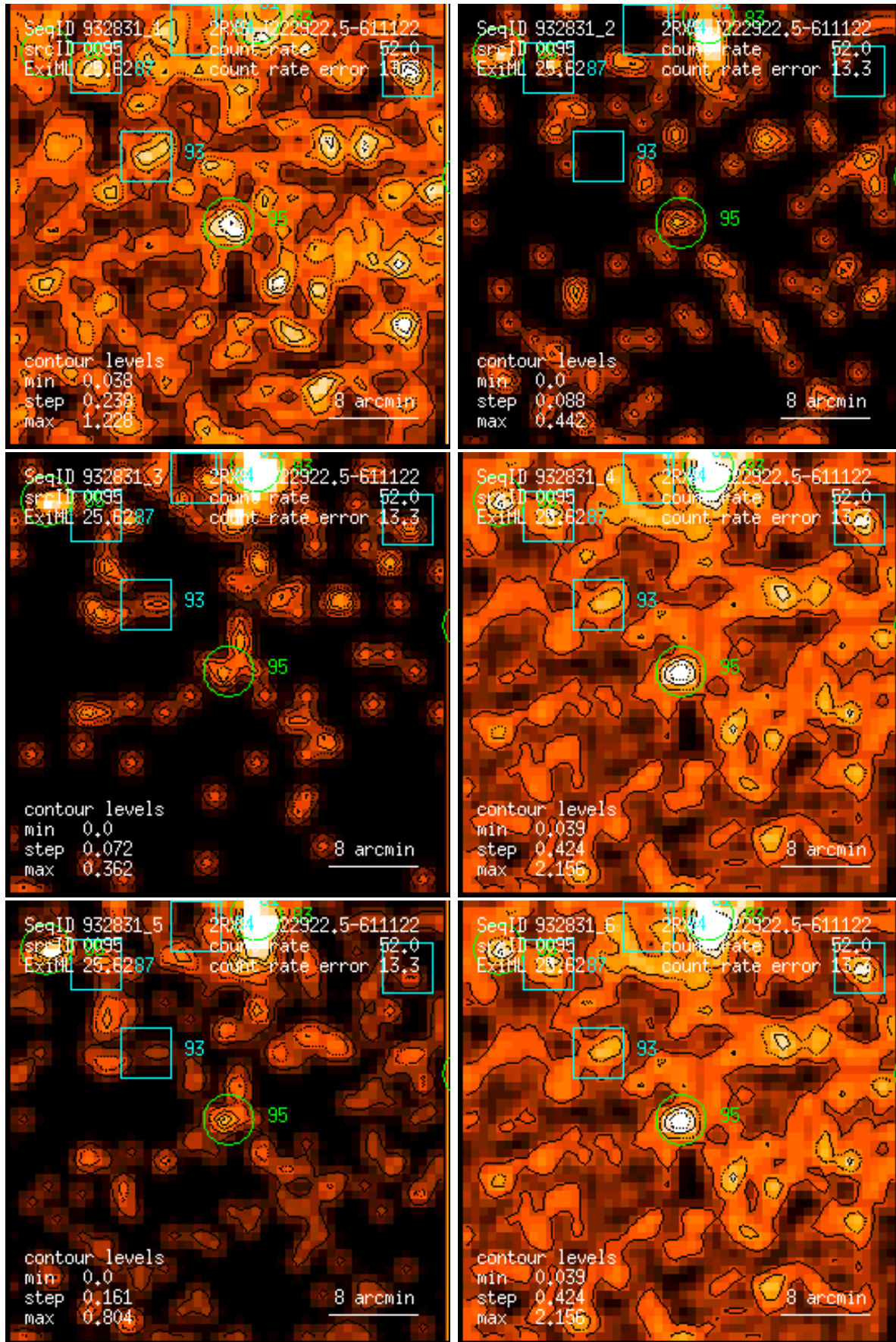
Figure 95: RASS 932831: detection 0095: band rate images, Gaussian filter: (1) PSPC channels 11 – 41, (2) 52 – 90, (3) 91 – 201, (4) 11 – 235, (5) 52 – 201, (6) 11 – 201. Broad band rates in counts/ks. Band rate contour levels in counts/ks/arcmin 2 .
