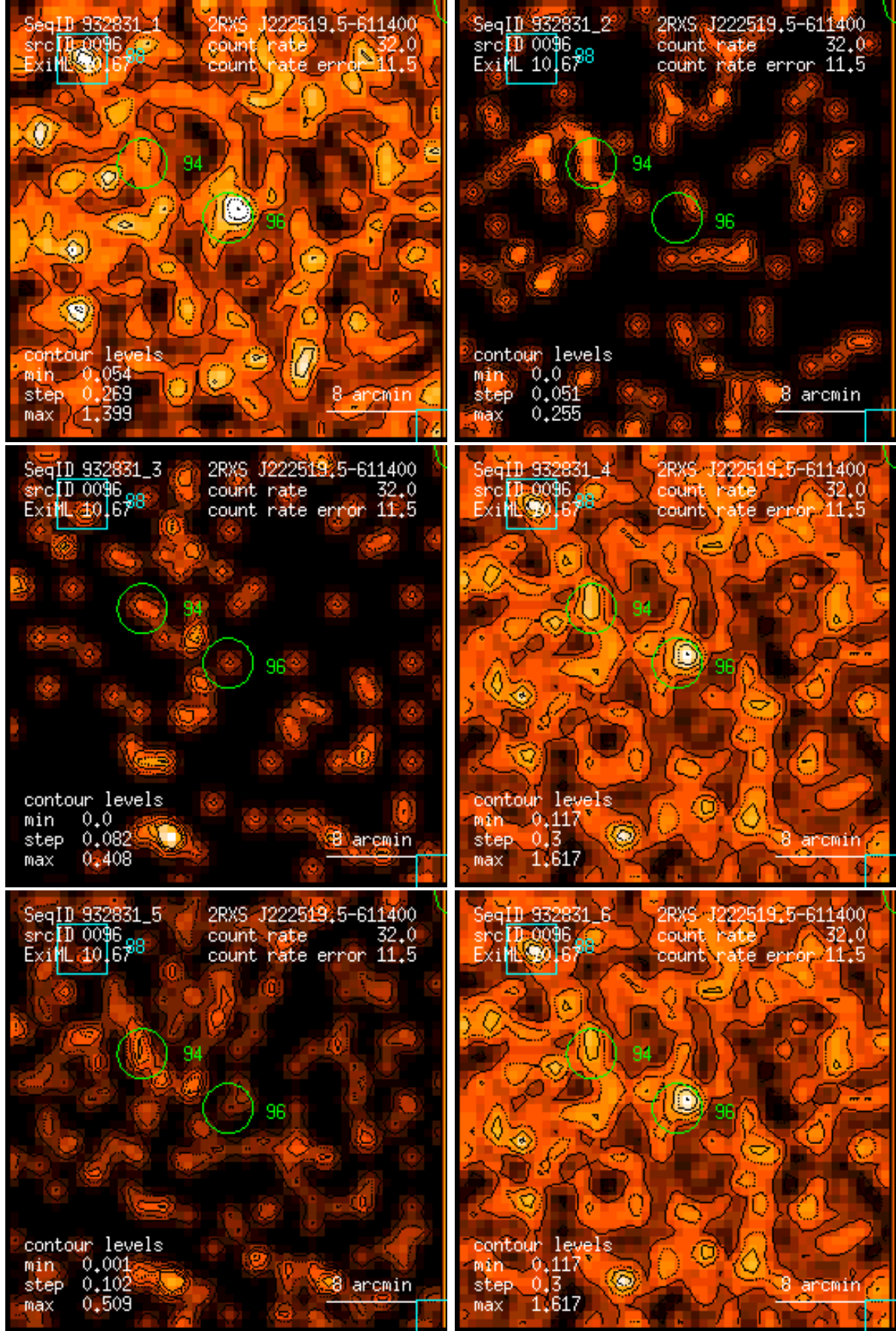
Figure 96: RASS 932831: detection 0096: band rate images, Gaussian filter: (1) PSPC channels 11 – 41, (2) 52 – 90, (3) 91 – 201, (4) 11 – 235, (5) 52 – 201, (6) 11 – 201. Broad band rates in counts/ks. Band rate contour levels in counts/ks/arcmin 2 .
