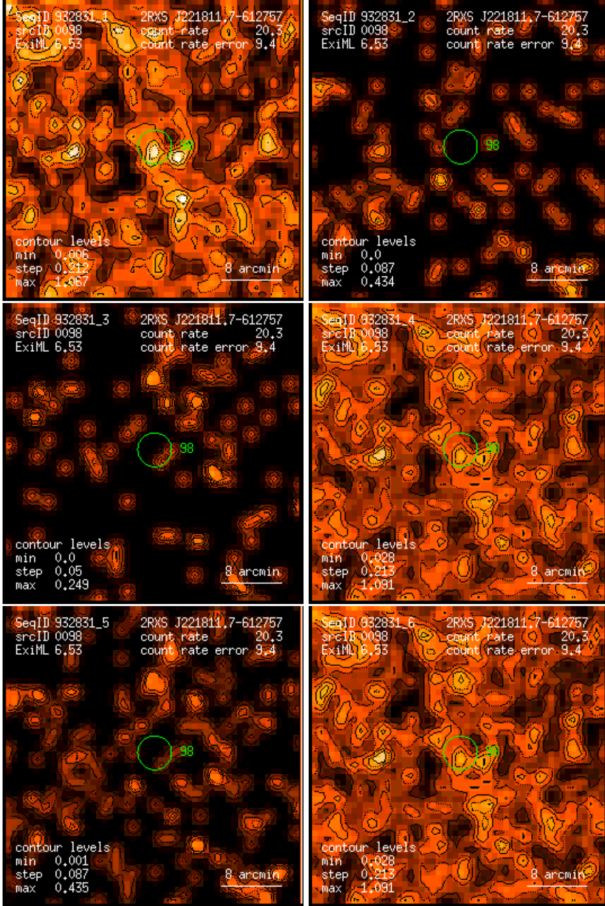
Figure 98: RASS 932831: detection 0098: band rate images, Gaussian filter: (1) PSPC channels 11 – 41, (2) 52 – 90, (3) 91 – 201, (4) 11 – 235, (5) 52 – 201, (6) 11 – 201. Broad band rates in counts/ks. Band rate contour levels in counts/ks/arcmin 2 .
