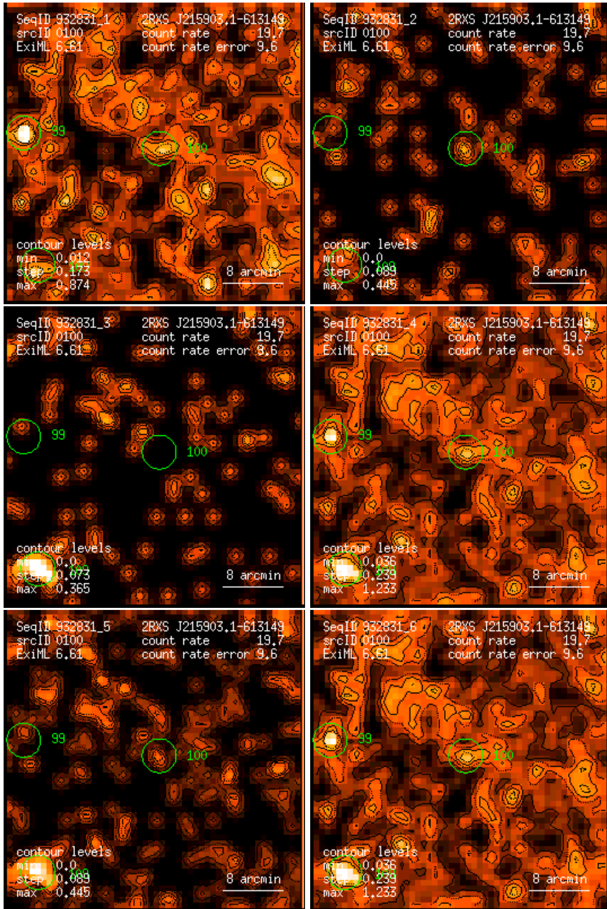
Figure 100: RASS 932831: detection 0100: band rate images, Gaussian filter: (1) PSPC channels 11 – 41, (2) 52 – 90, (3) 91 – 201, (4) 11 – 235, (5) 52 – 201, (6) 11 – 201. Broad band rates in counts/ks. Band rate contour levels in counts/ks/arcmin 2 .
