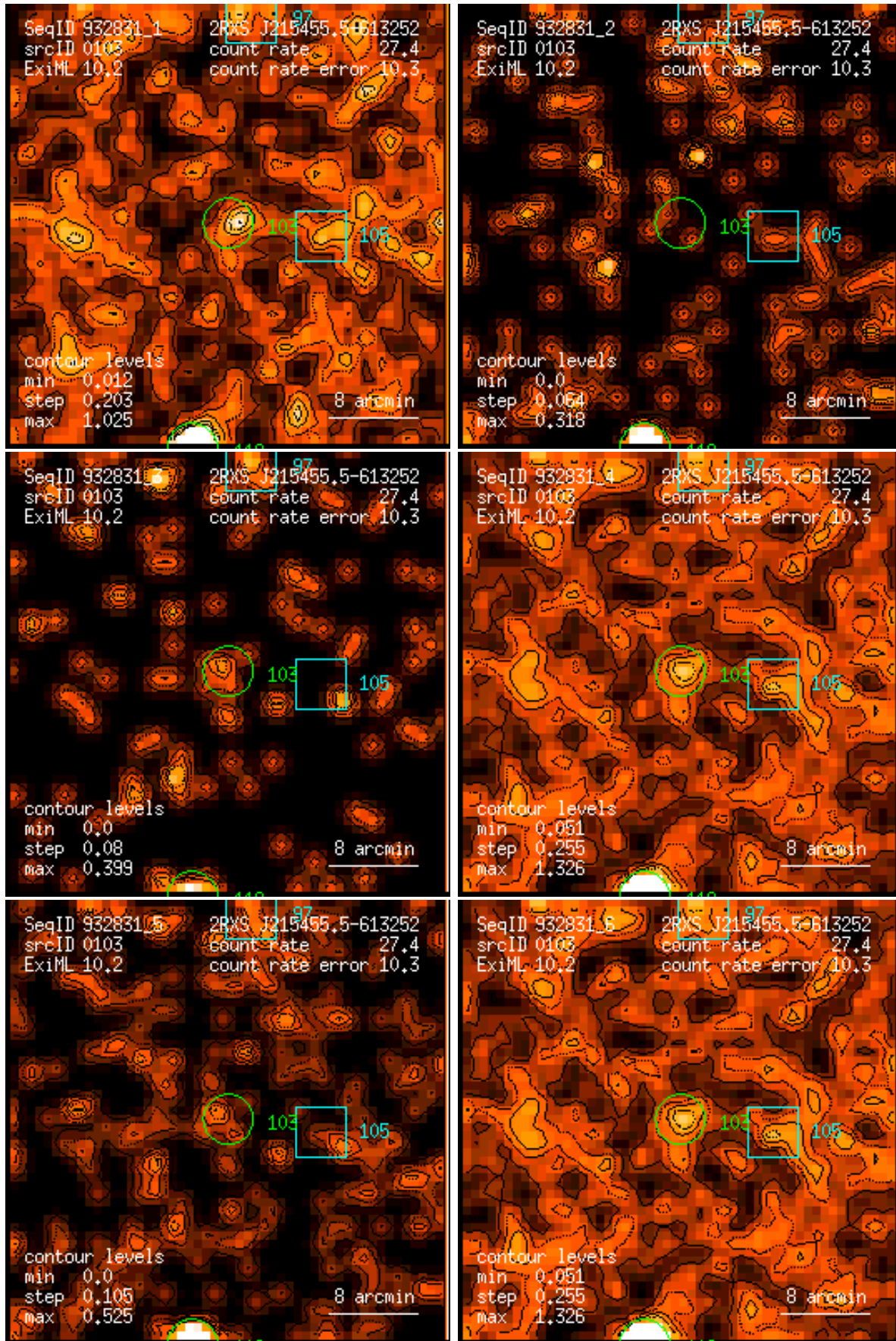
Figure 103: RASS 932831: detection 0103: band rate images, Gaussian filter: (1) PSPC channels 11 – 41, (2) 52 – 90, (3) 91 – 201, (4) 11 – 235, (5) 52 – 201, (6) 11 – 201. Broad band rates in counts/ks. Band rate contour levels in counts/ks/arcmin 2 .
