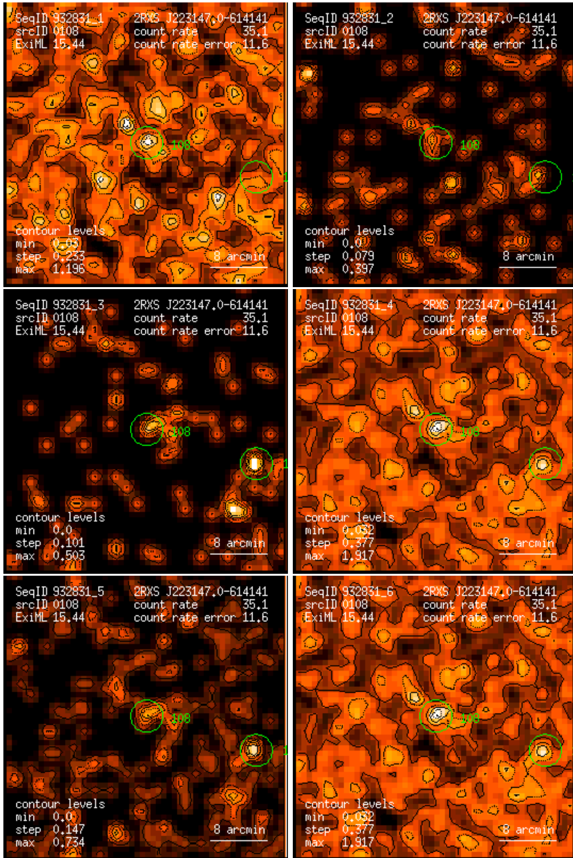
Figure 108: RASS 932831: detection 0108: band rate images, Gaussian filter: (1) PSPC channels 11 – 41, (2) 52 – 90, (3) 91 – 201, (4) 11 – 235, (5) 52 – 201, (6) 11 – 201. Broad band rates in counts/ks. Band rate contour levels in counts/ks/arcmin 2 .
