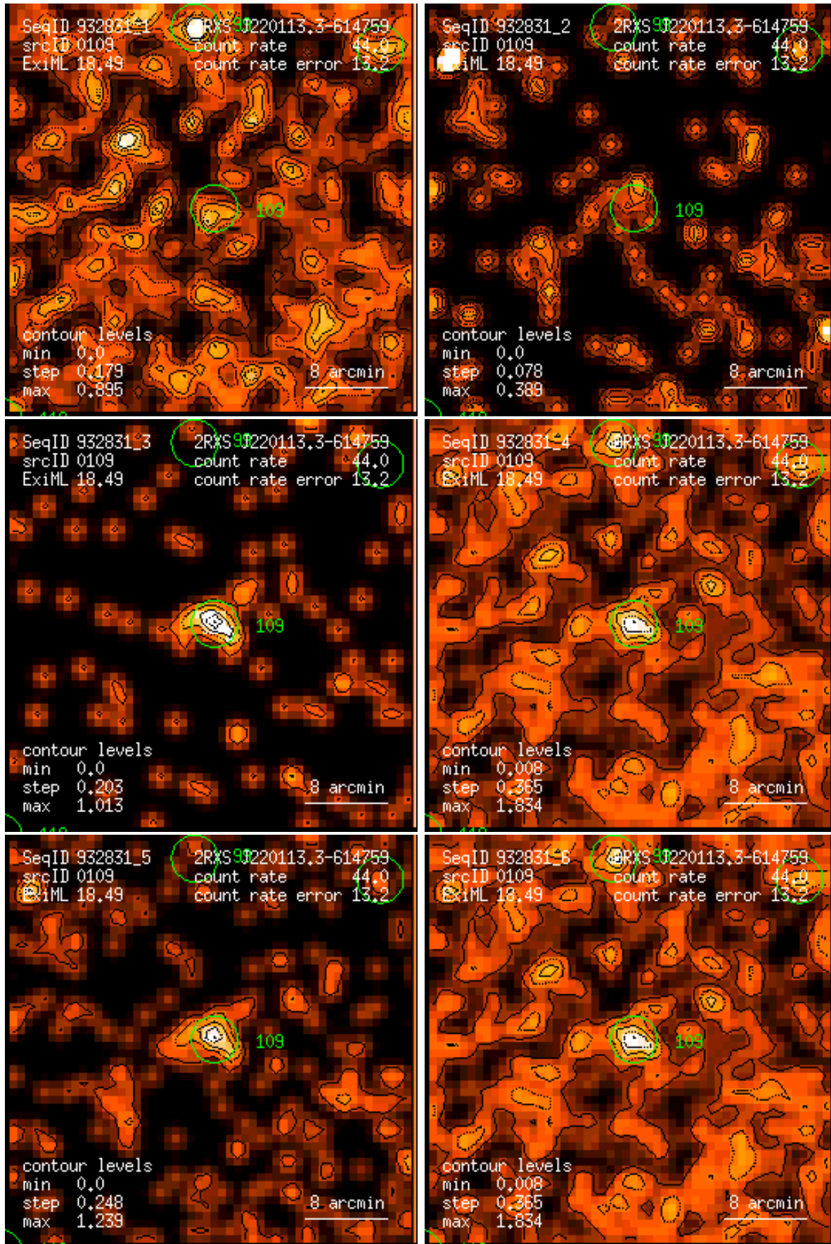
Figure 109: RASS 932831: detection 0109: band rate images, Gaussian filter: (1) PSPC channels 11 – 41, (2) 52 – 90, (3) 91 – 201, (4) 11 – 235, (5) 52 – 201, (6) 11 – 201. Broad band rates in counts/ks. Band rate contour levels in counts/ks/arcmin 2 .
