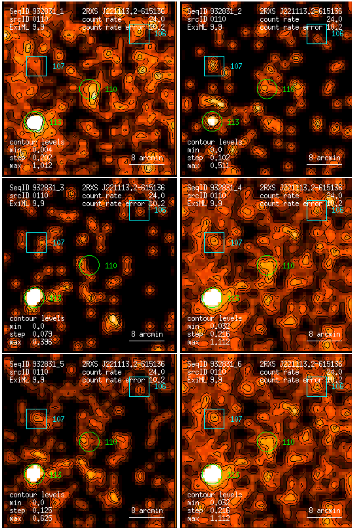
Figure 110: RASS 932831: detection 0110: band rate images, Gaussian filter: (1) PSPC channels 11 – 41, (2) 52 – 90, (3) 91 – 201, (4) 11 – 235, (5) 52 – 201, (6) 11 – 201. Broad band rates in counts/ks. Band rate contour levels in counts/ks/arcmin 2 .
