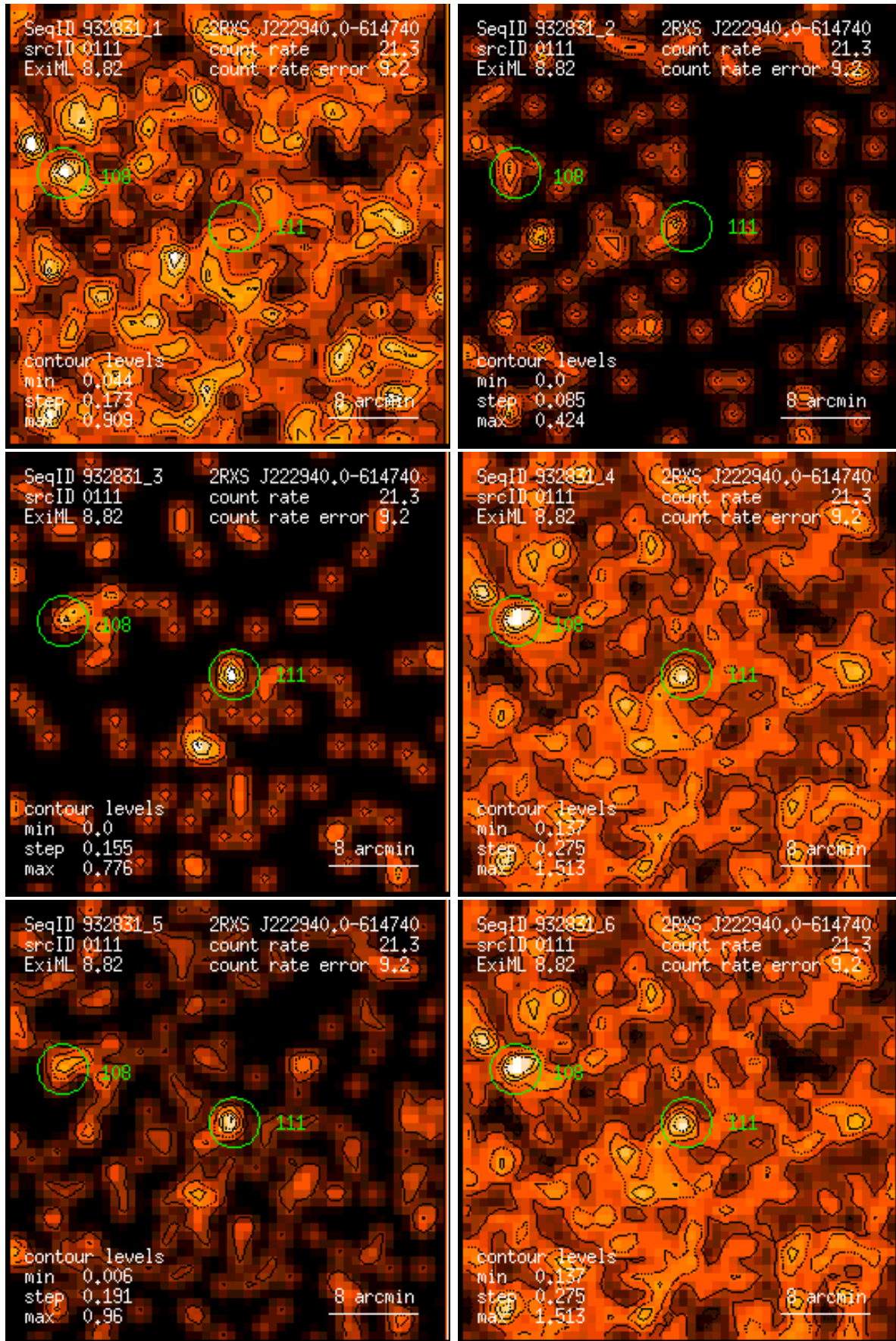
Figure 111: RASS 932831: detection 0111: band rate images, Gaussian filter: (1) PSPC channels 11 – 41, (2) 52 – 90, (3) 91 – 201, (4) 11 – 235, (5) 52 – 201, (6) 11 – 201. Broad band rates in counts/ks. Band rate contour levels in counts/ks/arcmin 2 .
