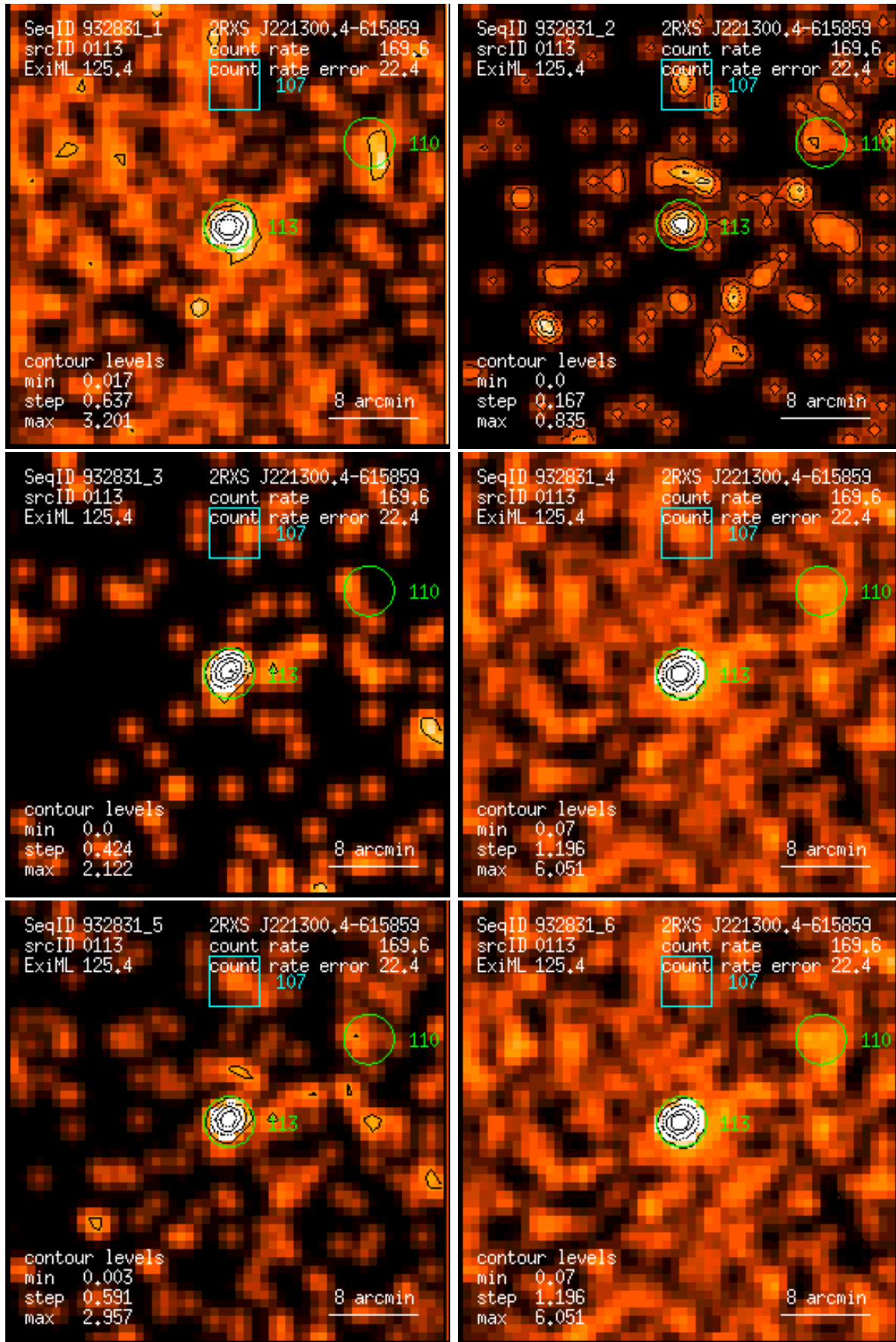
Figure 113: RASS 932831: detection 0113: band rate images, Gaussian filter: (1) PSPC channels 11 – 41, (2) 52 – 90, (3) 91 – 201, (4) 11 – 235, (5) 52 – 201, (6) 11 – 201. Broad band rates in counts/ks. Band rate contour levels in counts/ks/arcmin 2 .
