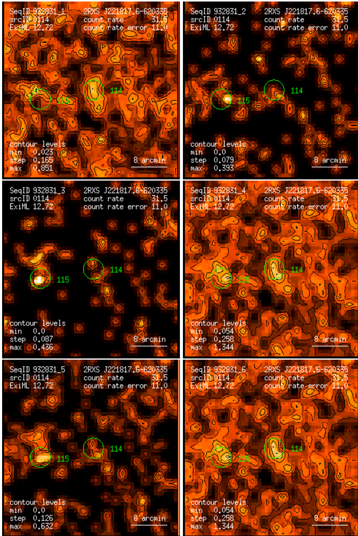
Figure 114: RASS 932831: detection 0114: band rate images, Gaussian filter: (1) PSPC channels 11 – 41, (2) 52 – 90, (3) 91 – 201, (4) 11 – 235, (5) 52 – 201, (6) 11 – 201. Broad band rates in counts/ks. Band rate contour levels in counts/ks/arcmin 2 .
