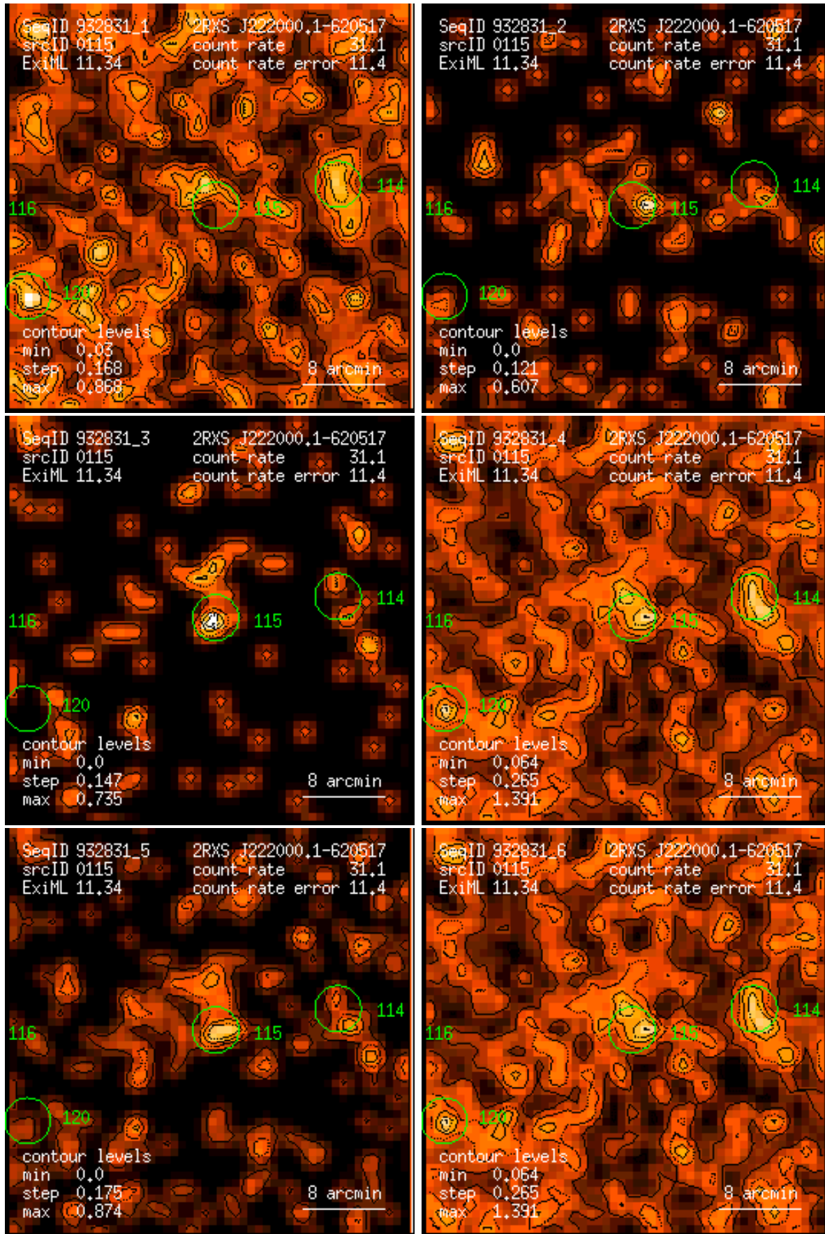
Figure 115: RASS 932831: detection 0115: band rate images, Gaussian filter: (1) PSPPC channels 11 – 41, (2) 52 – 90, (3) 91 – 201, (4) 11 – 235, (5) 52 – 201, (6) 11 – 201. Broad band rates in counts/ks. Band rate contour levels in counts/ks/arcmin 2 .
