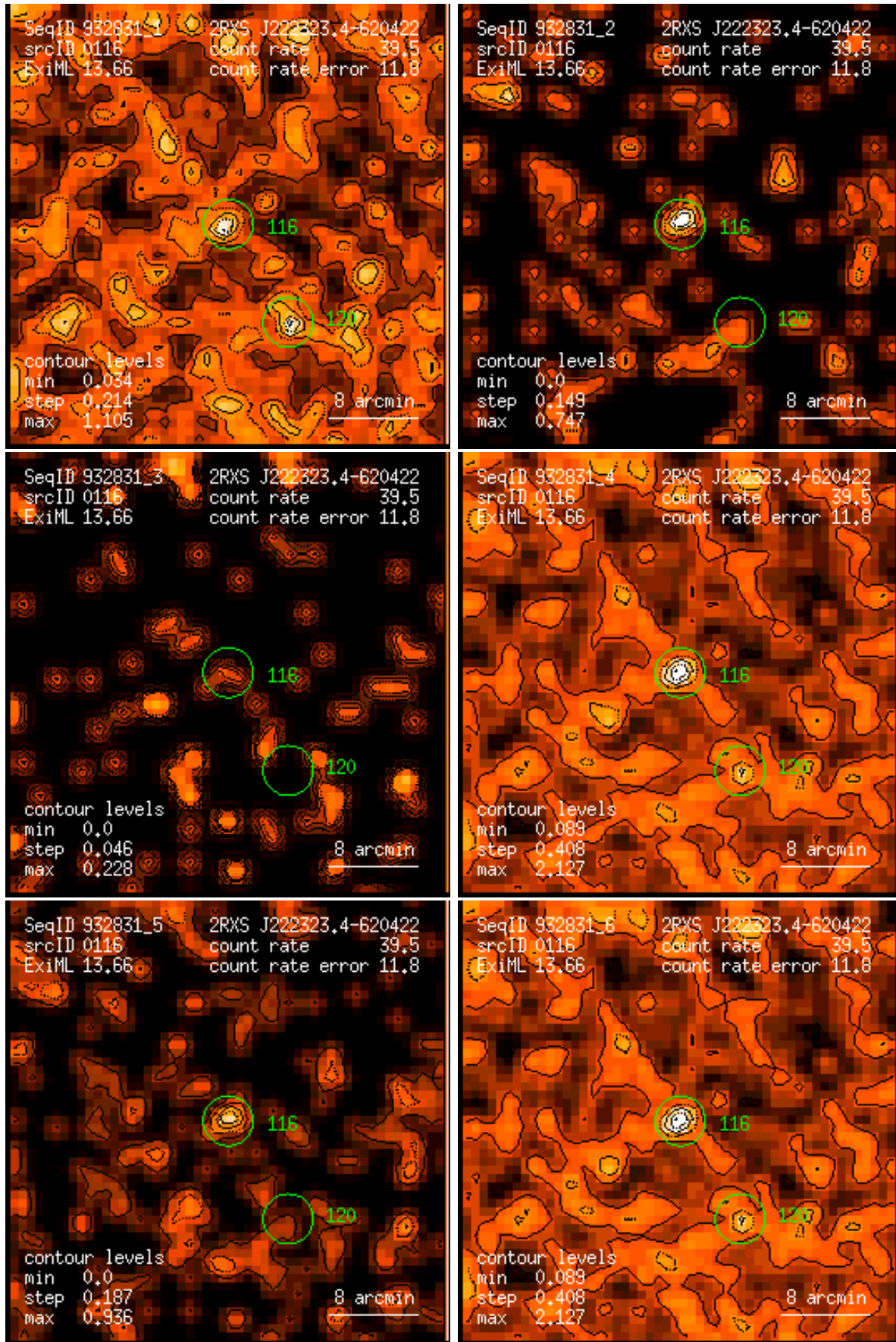
Figure 116: RASS 932831: detection 0116: band rate images, Gaussian filter: (1) PSPC channels 11 – 41, (2) 52 – 90, (3) 91 – 201, (4) 11 – 235, (5) 52 – 201, (6) 11 – 201. Broad band rates in counts/ks. Band rate contour levels in counts/ks/arcmin 2 .
