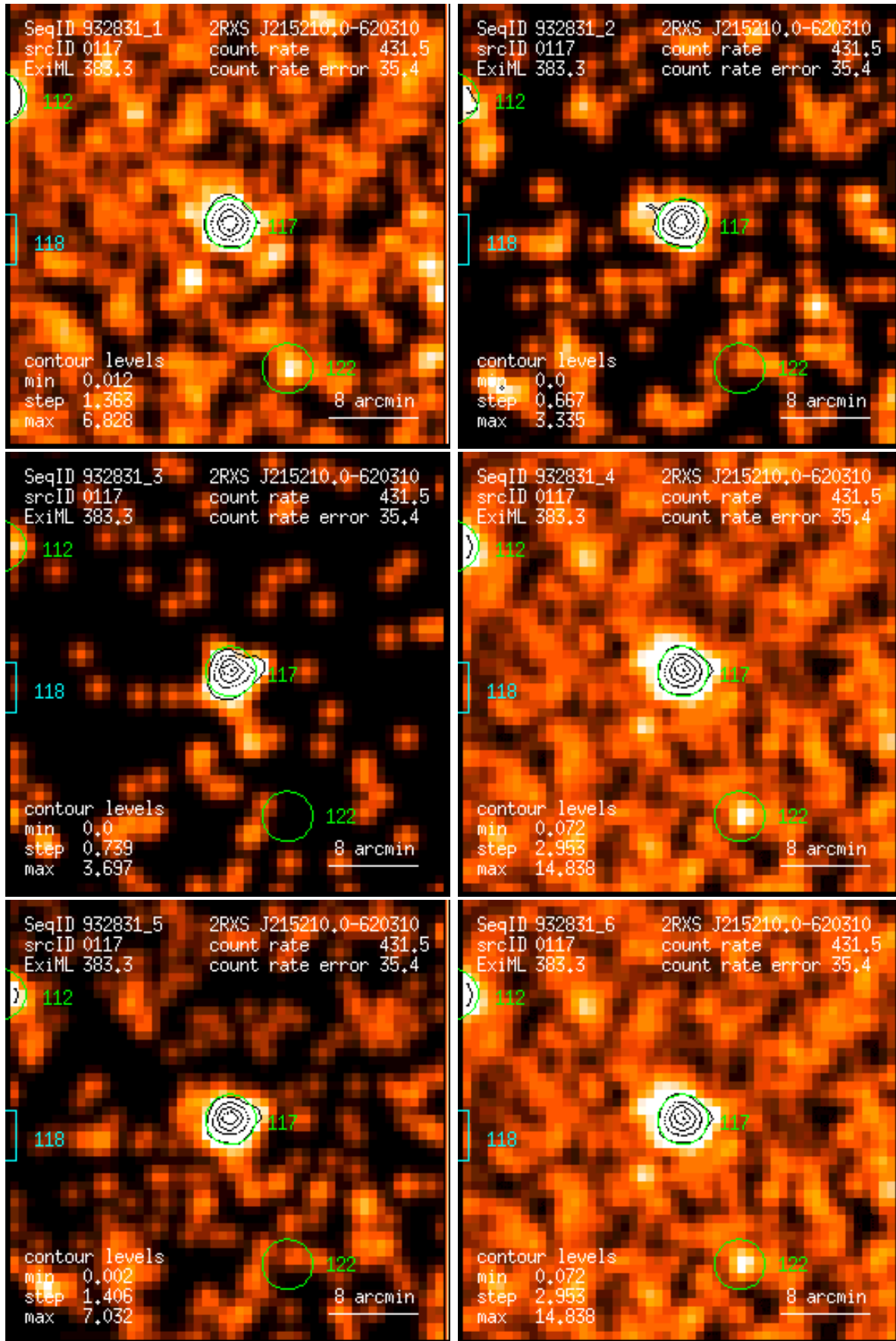
Figure 117: RASS 932831: detection 0117: band rate images, Gaussian filter: (1) PSPC channels 11 – 41, (2) 52 – 90, (3) 91 – 201, (4) 11 – 235, (5) 52 – 201, (6) 11 – 201. Broad band rates in counts/ks. Band rate contour levels in counts/ks/arcmin 2 .
