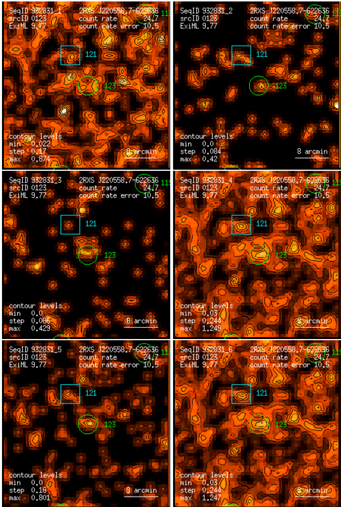
Figure 123: RASS 932831: detection 0123: band rate images, Gaussian filter: (1) PSPC channels 11 – 41, (2) 52 – 90, (3) 91 – 201, (4) 11 – 235, (5) 52 – 201, (6) 11 – 201. Broad band rates in counts/ks. Band rate contour levels in counts/ks/arcmin 2 .
