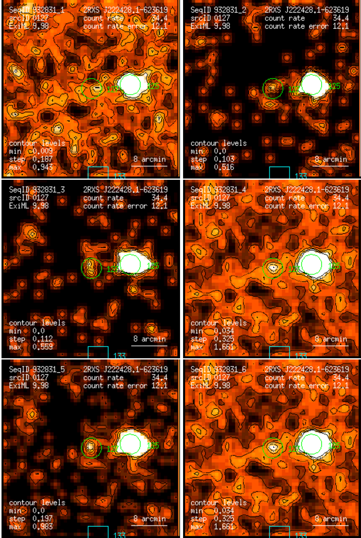
Figure 127: RASS 932831: detection 0127: band rate images, Gaussian filter: (1) PSPC channels 11 – 41, (2) 52 – 90, (3) 91 – 201, (4) 11 – 235, (5) 52 – 201, (6) 11 – 201. Broad band rates in counts/ks. Band rate contour levels in counts/ks/arcmin 2 .
