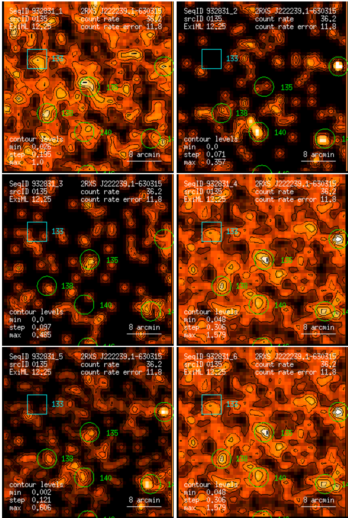
Figure 135: RASS 932831: detection 0135: band rate images, Gaussian filter: (1) PSPC channels 11 – 41, (2) 52 – 90, (3) 91 – 201, (4) 11 – 235, (5) 52 – 201, (6) 11 – 201. Broad band rates in counts/ks. Band rate contour levels in counts/ks/arcmin 2 .
