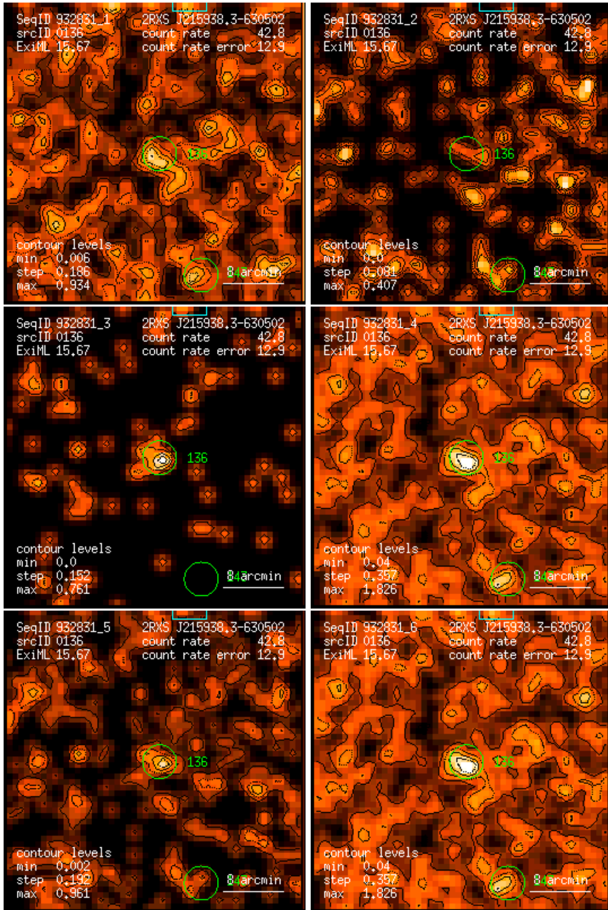
Figure 136: RASS 932831: detection 0136: band rate images, Gaussian filter: (1) PSPC channels 11 – 41, (2) 52 – 90, (3) 91 – 201, (4) 11 – 235, (5) 52 – 201, (6) 11 – 201. Broad band rates in counts/ks. Band rate contour levels in counts/ks/arcmin 2 .
