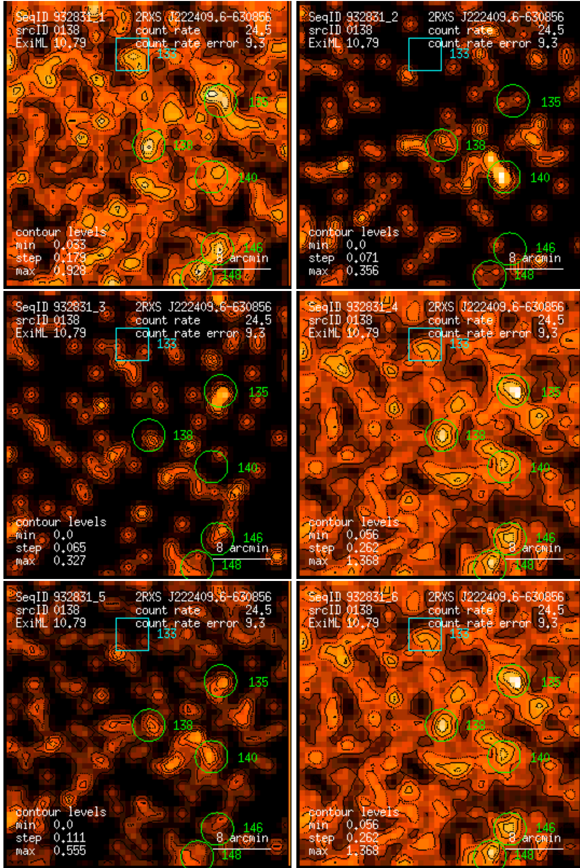
Figure 138: RASS 932831: detection 0138: band rate images, Gaussian filter: (1) PSPC channels 11 – 41, (2) 52 – 90, (3) 91 – 201, (4) 11 – 235, (5) 52 – 201, (6) 11 – 201. Broad band rates in counts/ks. Band rate contour levels in counts/ks/arcmin 2 .
