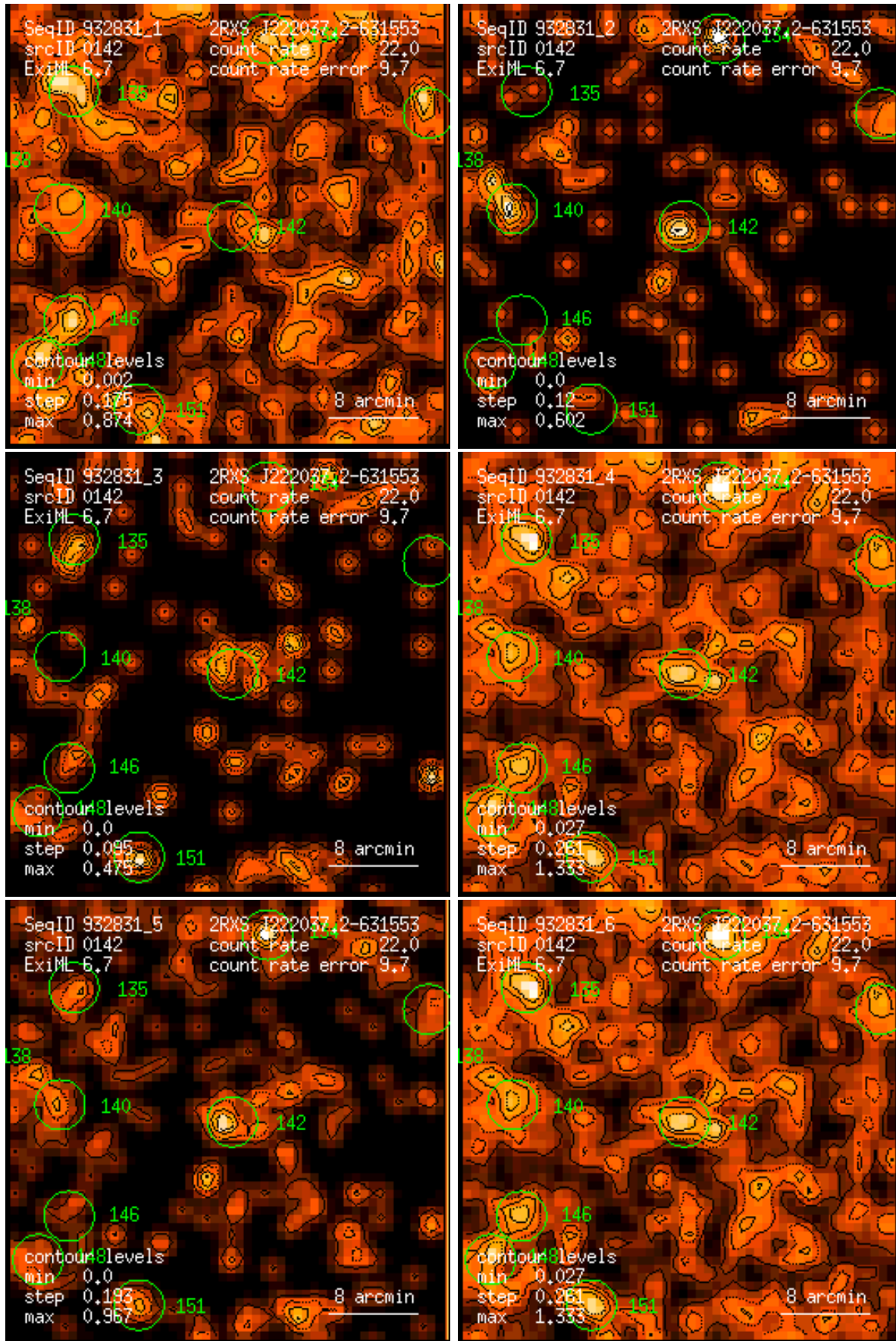
Figure 142: RASS 932831: detection 0142: band rate images, Gaussian filter: (1) PSPC channels 11 – 41, (2) 52 – 90, (3) 91 – 201, (4) 11 – 235, (5) 52 – 201, (6) 11 – 201. Broad band rates in counts/ks. Band rate contour levels in counts/ks/arcmin 2 .
