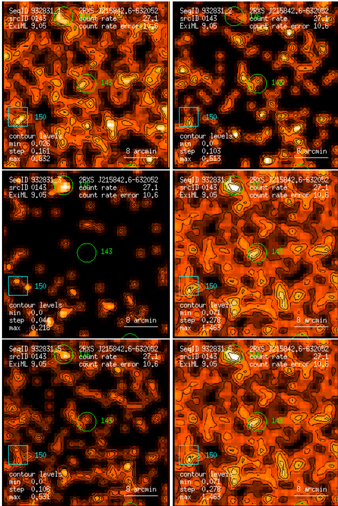
Figure 143: RASS 932831: detection 0143: band rate images, Gaussian filter: (1) PSPC channels 11 – 41, (2) 52 – 90, (3) 91 – 201, (4) 11 – 235, (5) 52 – 201, (6) 11 – 201. Broad band rates in counts/ks. Band rate contour levels in counts/ks/arcmin 2 .
