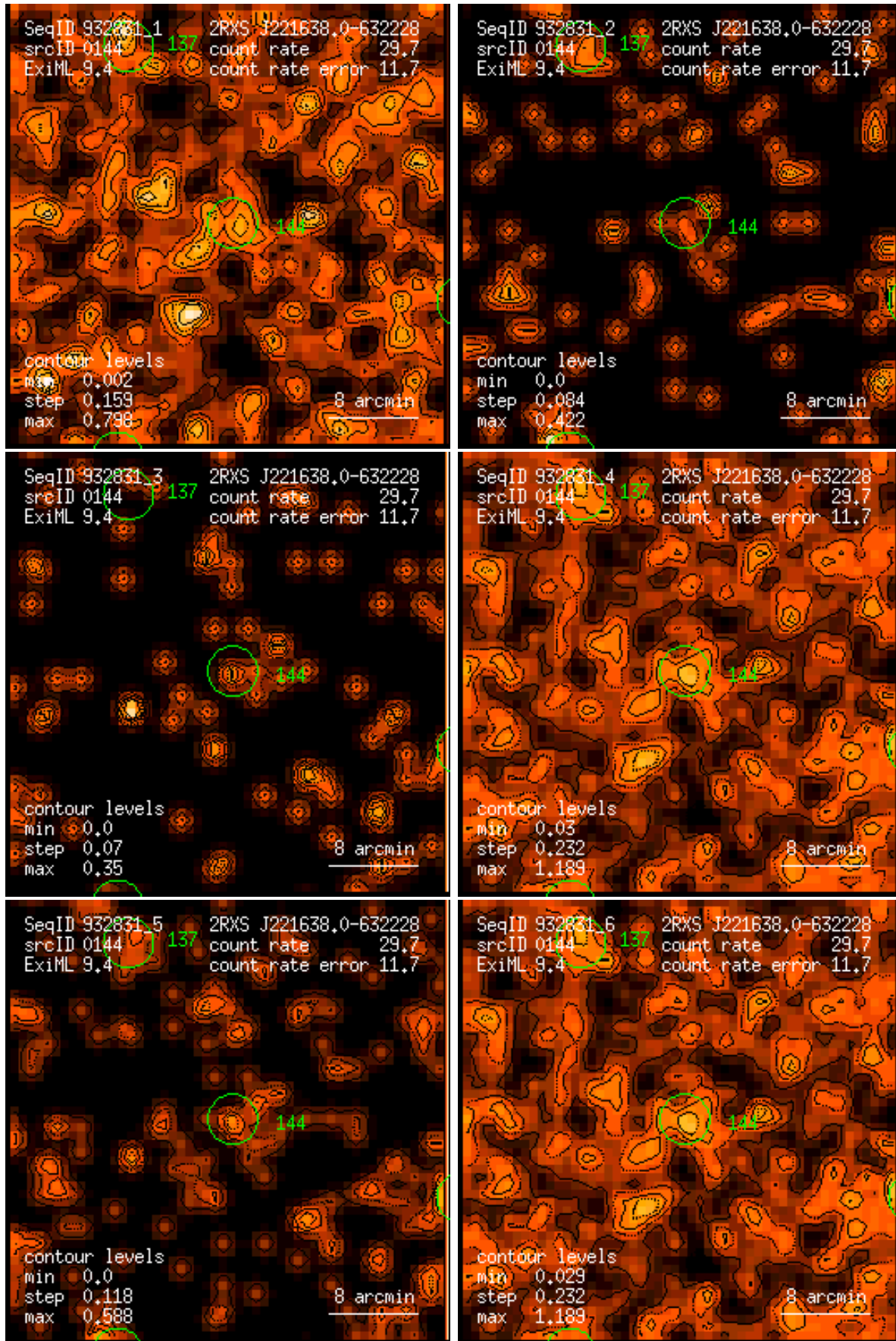
Figure 144: RASS 932831: detection 0144: band rate images, Gaussian filter: (1) PSPC channels 11 – 41, (2) 52 – 90, (3) 91 – 201, (4) 11 – 235, (5) 52 – 201, (6) 11 – 201. Broad band rates in counts/ks. Band rate contour levels in counts/ks/arcmin 2 .
