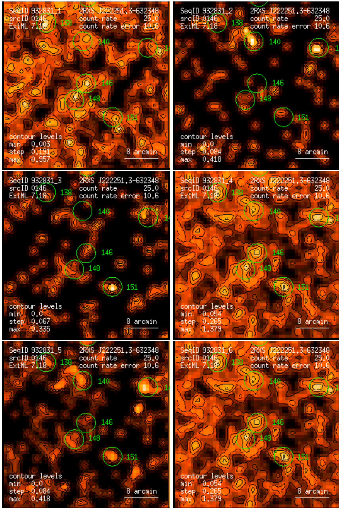
Figure 146: RASS 932831: detection 0146: band rate images, Gaussian filter: (1) PSPPC channels 11 – 41, (2) 52 – 90, (3) 91 – 201, (4) 11 – 235, (5) 52 – 201, (6) 11 – 201. Broad band rates in counts/ks. Band rate contour levels in counts/ks/arcmin 2 .
