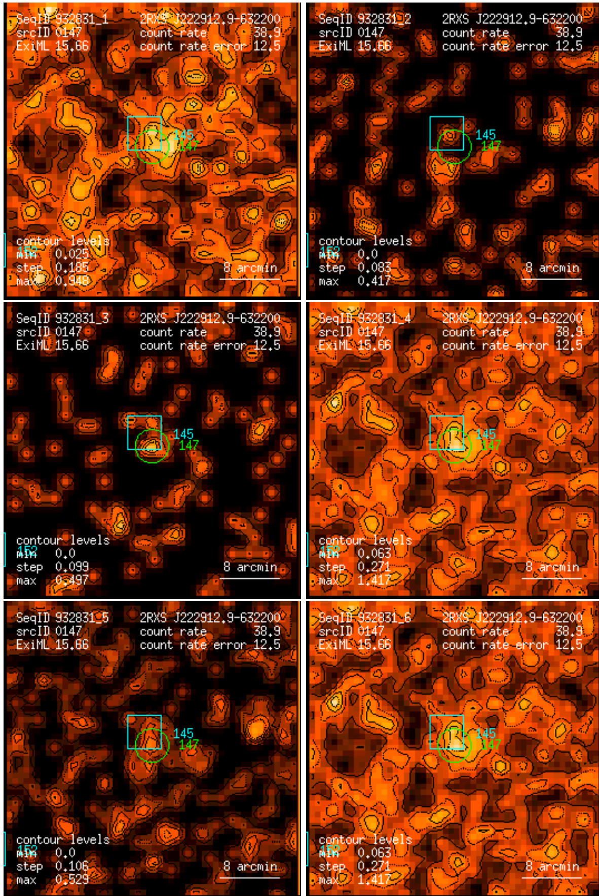
Figure 147: RASS 932831: detection 0147: band rate images, Gaussian filter: (1) PSPC channels 11 – 41, (2) 52 – 90, (3) 91 – 201, (4) 11 – 235, (5) 52 – 201, (6) 11 – 201. Broad band rates in counts/ks. Band rate contour levels in counts/ks/arcmin 2 .
