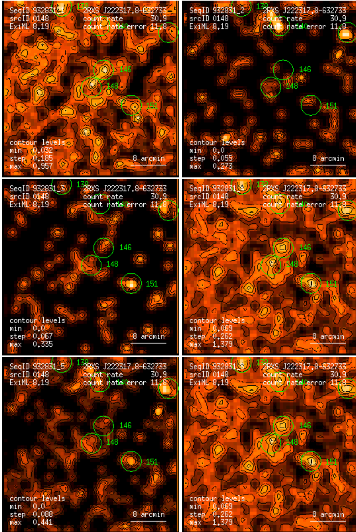
Figure 148: RASS 932831: detection 0148: band rate images, Gaussian filter: (1) PSPC channels 11 – 41, (2) 52 – 90, (3) 91 – 201, (4) 11 – 235, (5) 52 – 201, (6) 11 – 201. Broad band rates in counts/ks. Band rate contour levels in counts/ks/arcmin 2 .
