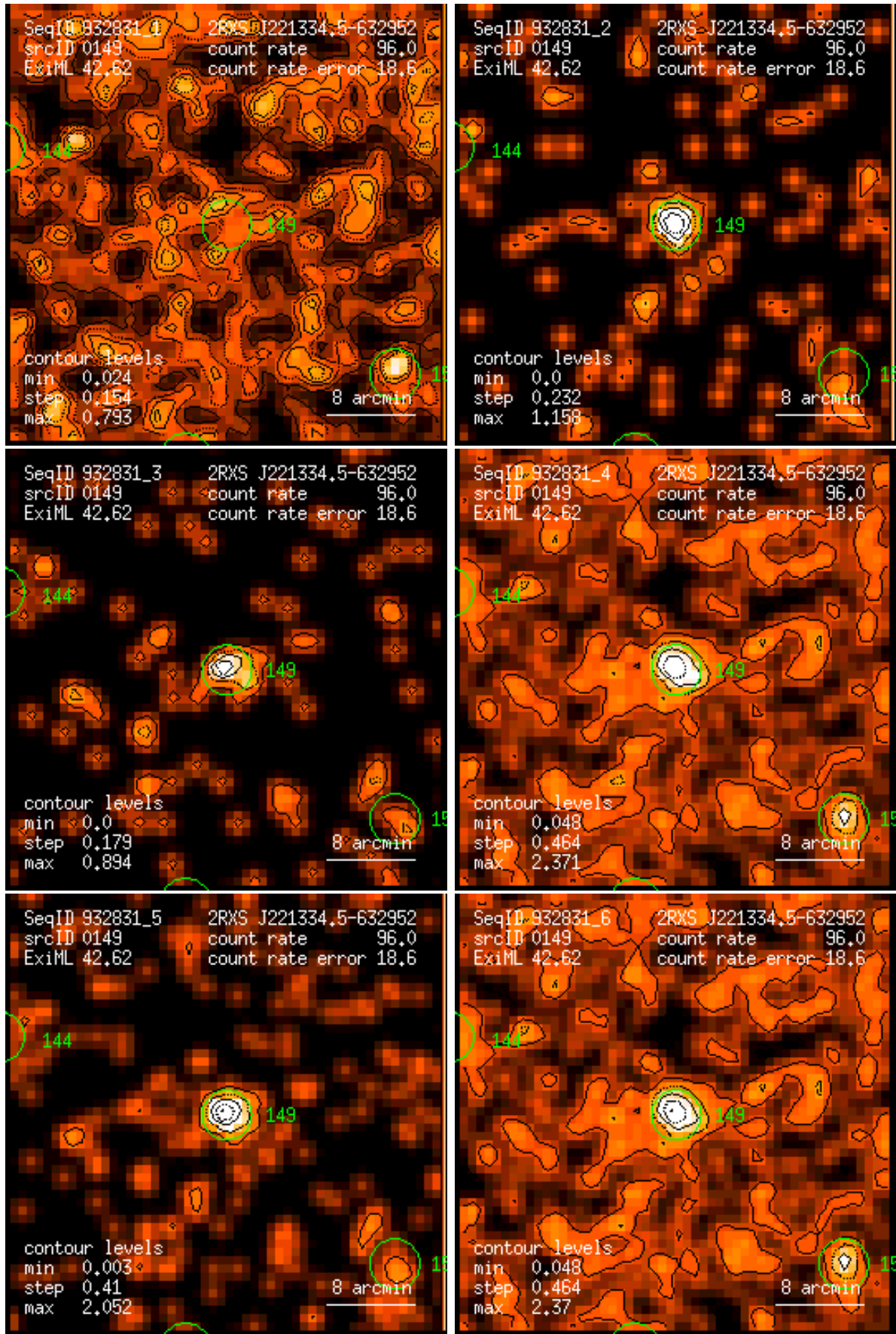
Figure 149: RASS 932831: detection 0149: band rate images, Gaussian filter: (1) PSPC channels 11 – 41, (2) 52 – 90, (3) 91 – 201, (4) 11 – 235, (5) 52 – 201, (6) 11 – 201. Broad band rates in counts/ks. Band rate contour levels in counts/ks/arcmin 2 .
