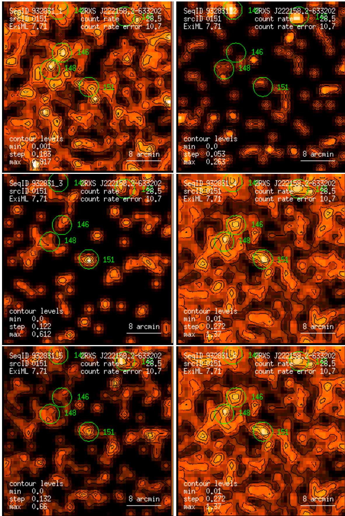
Figure 151: RASS 932831: detection 0151: band rate images, Gaussian filter: (1) PSPC channels 11 – 41, (2) 52 – 90, (3) 91 – 201, (4) 11 – 235, (5) 52 – 201, (6) 11 – 201. Broad band rates in counts/ks. Band rate contour levels in counts/ks/arcmin 2 .
