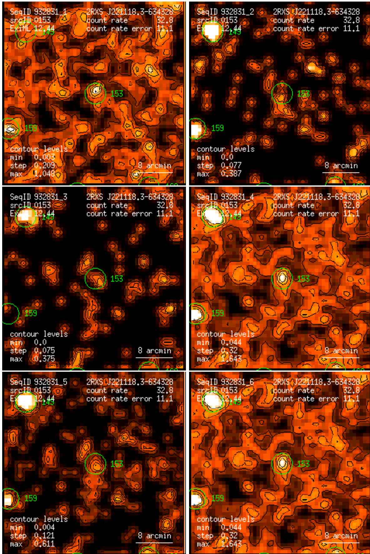
Figure 153: RASS 932831: detection 0153: band rate images, Gaussian filter: (1) PSPC channels 11 – 41, (2) 52 – 90, (3) 91 – 201, (4) 11 – 235, (5) 52 – 201, (6) 11 – 201. Broad band rates in counts/ks. Band rate contour levels in counts/ks/arcmin 2 .
