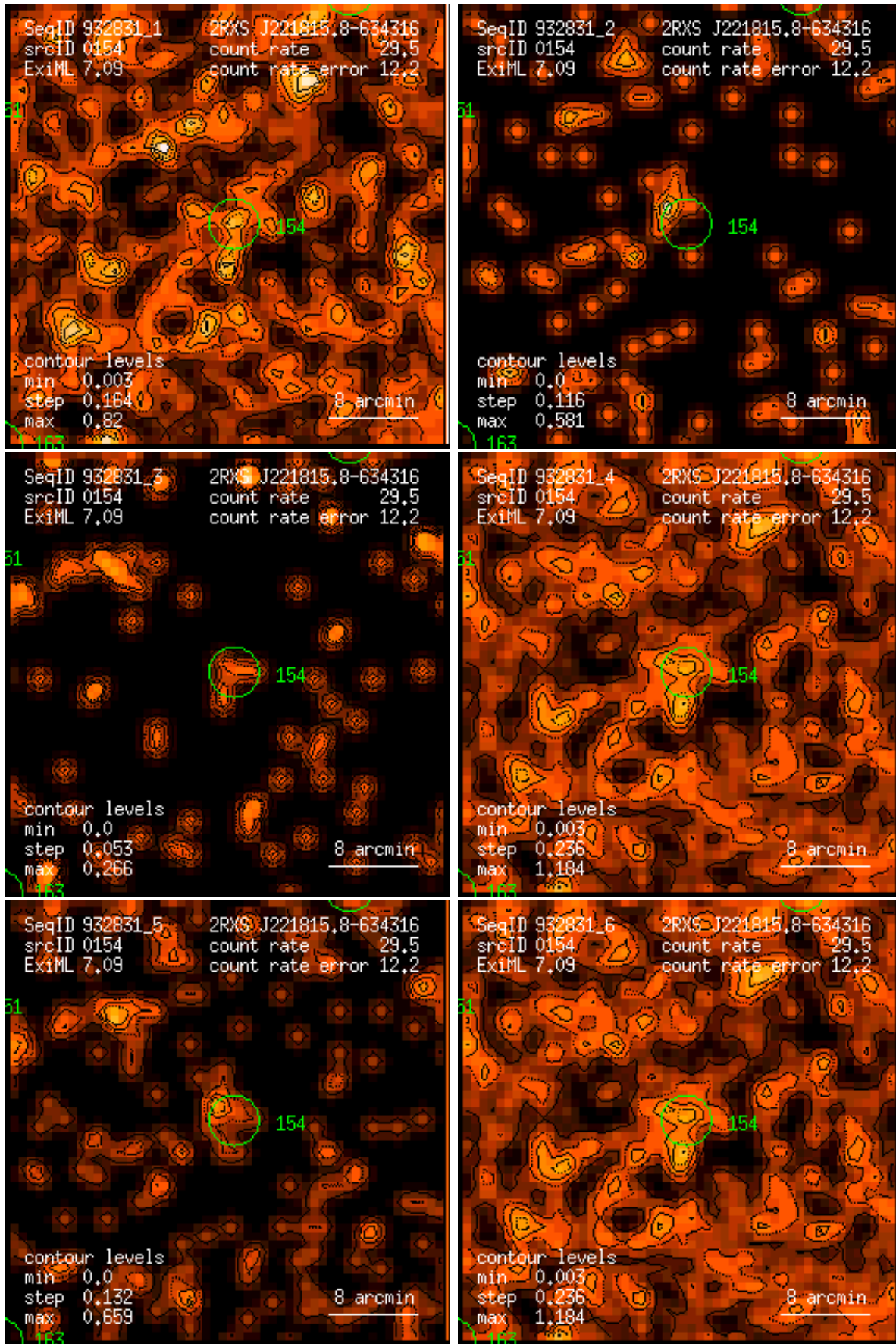
Figure 154: RASS 932831: detection 0154: band rate images, Gaussian filter: (1) PSPC channels 11 – 41, (2) 52 – 90, (3) 91 – 201, (4) 11 – 235, (5) 52 – 201, (6) 11 – 201. Broad band rates in counts/ks. Band rate contour levels in counts/ks/arcmin 2 .
