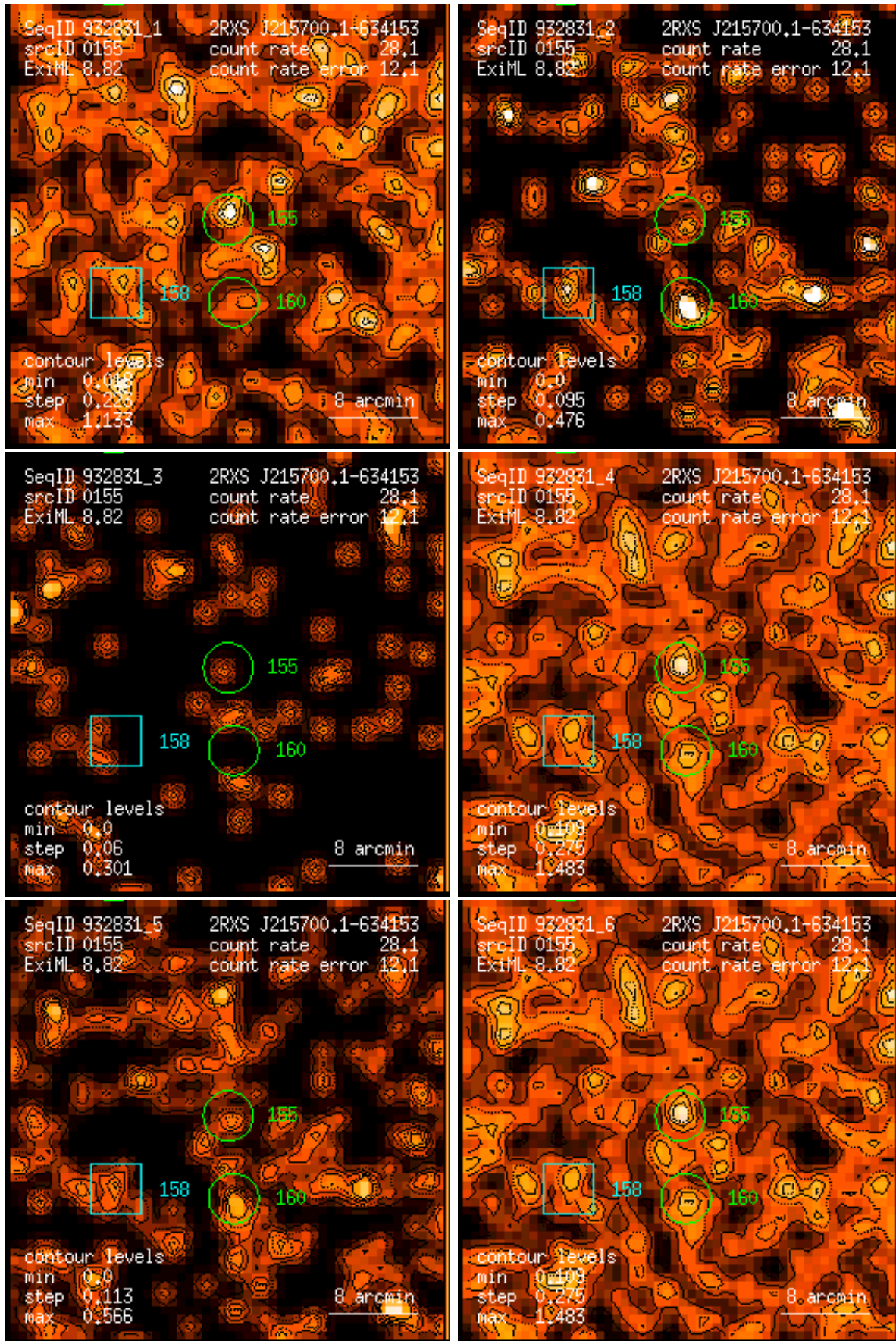
Figure 155: RASS 932831: detection 0155: band rate images, Gaussian filter: (1) PSPC channels 11 – 41, (2) 52 – 90, (3) 91 – 201, (4) 11 – 235, (5) 52 – 201, (6) 11 – 201. Broad band rates in counts/ks. Band rate contour levels in counts/ks/arcmin 2 .
