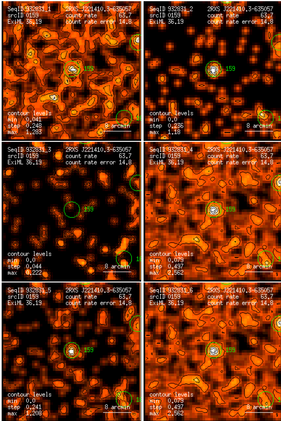
Figure 159: RASS 932831: detection 0159: band rate images, Gaussian filter: (1) PSPC channels 11 – 41, (2) 52 – 90, (3) 91 – 201, (4) 11 – 235, (5) 52 – 201, (6) 11 – 201. Broad band rates in counts/ks. Band rate contour levels in counts/ks/arcmin 2 .
