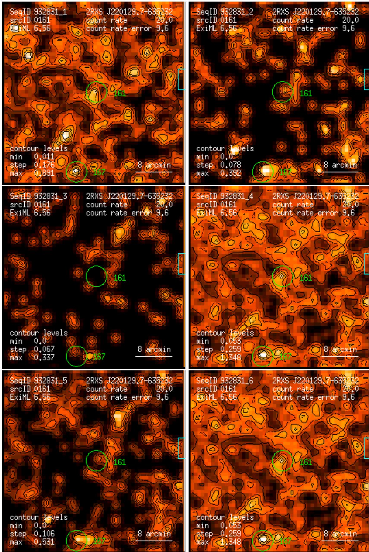
Figure 161: RASS 932831: detection 0161: band rate images, Gaussian filter: (1) PSPC channels 11 – 41, (2) 52 – 90, (3) 91 – 201, (4) 11 – 235, (5) 52 – 201, (6) 11 – 201. Broad band rates in counts/ks. Band rate contour levels in counts/ks/arcmin 2 .
