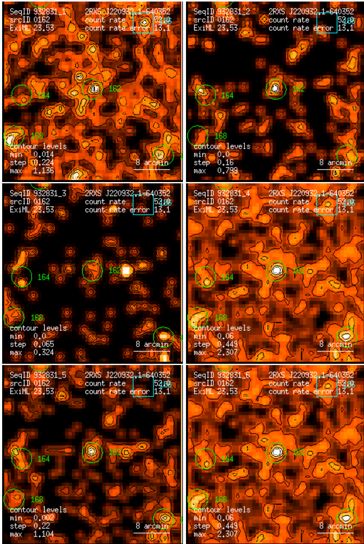
Figure 162: RASS 932831: detection 0162: band rate images, Gaussian filter: (1) PSPC channels 11 – 41, (2) 52 – 90, (3) 91 – 201, (4) 11 – 235, (5) 52 – 201, (6) 11 – 201. Broad band rates in counts/ks. Band rate contour levels in counts/ks/arcmin 2 .
