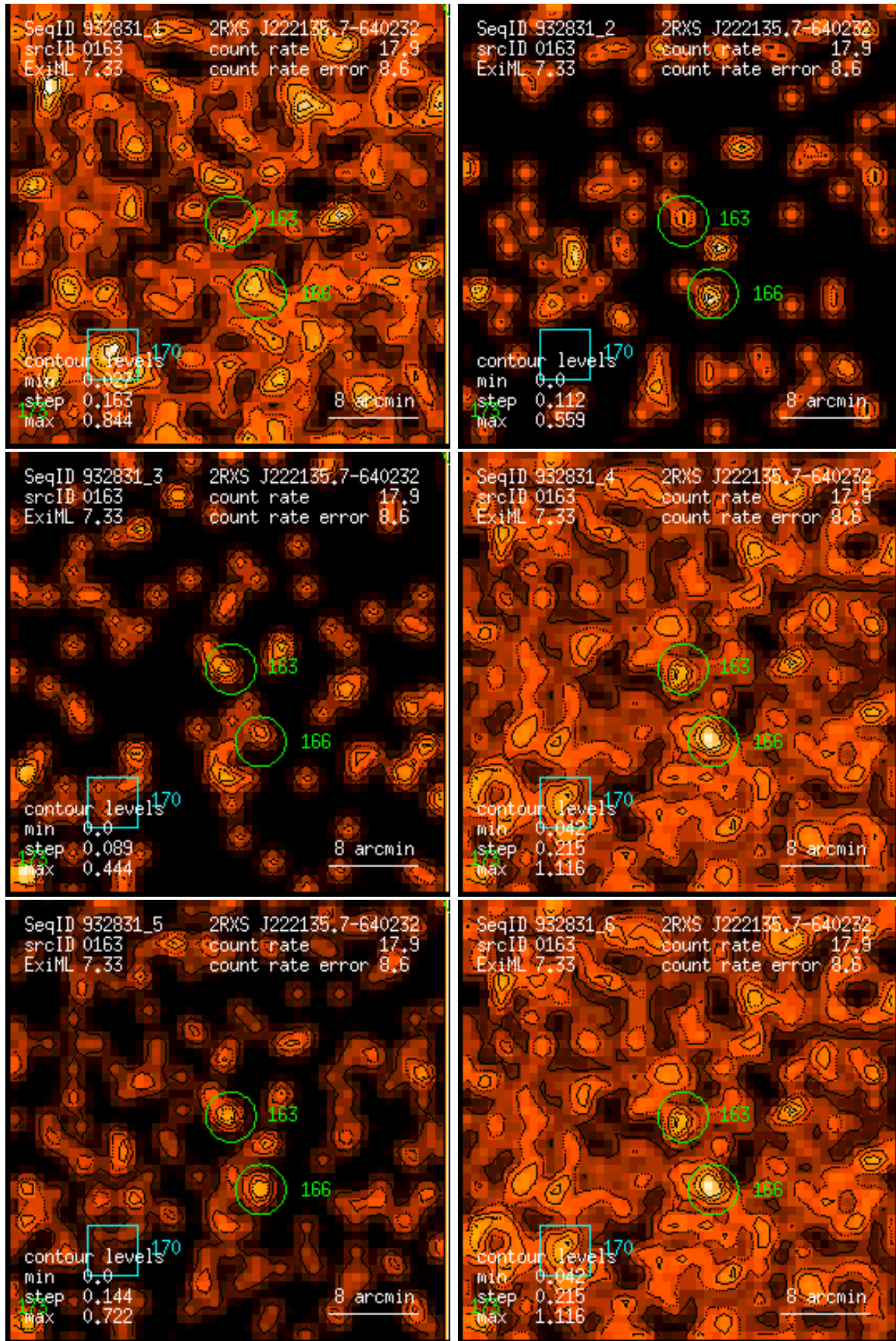
Figure 163: RASS 932831: detection 0163: band rate images, Gaussian filter: (1) PSPC channels 11 – 41, (2) 52 – 90, (3) 91 – 201, (4) 11 – 235, (5) 52 – 201, (6) 11 – 201. Broad band rates in counts/ks. Band rate contour levels in counts/ks/arcmin 2 .
