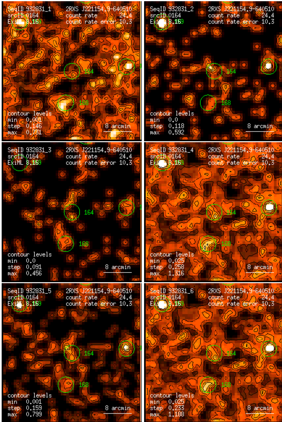
Figure 164: RASS 932831: detection 0164: band rate images, Gaussian filter: (1) PSPC channels 11 – 41, (2) 52 – 90, (3) 91 – 201, (4) 11 – 235, (5) 52 – 201, (6) 11 – 201. Broad band rates in counts/ks. Band rate contour levels in counts/ks/arcmin 2 .
