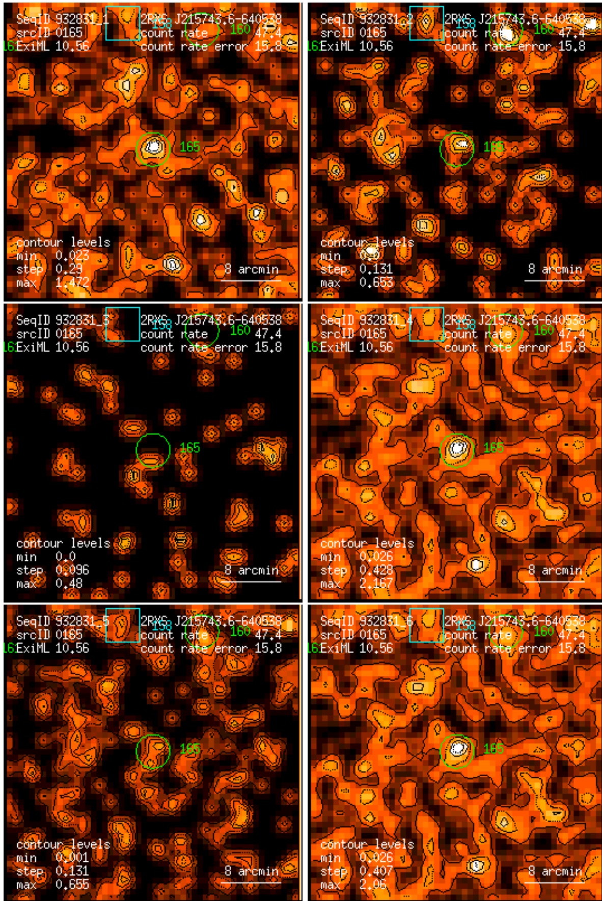
Figure 165: RASS 932831: detection 0165: band rate images, Gaussian filter: (1) PSPC channels 11 – 41, (2) 52 – 90, (3) 91 – 201, (4) 11 – 235, (5) 52 – 201, (6) 11 – 201. Broad band rates in counts/ks. Band rate contour levels in counts/ks/arcmin 2 .
