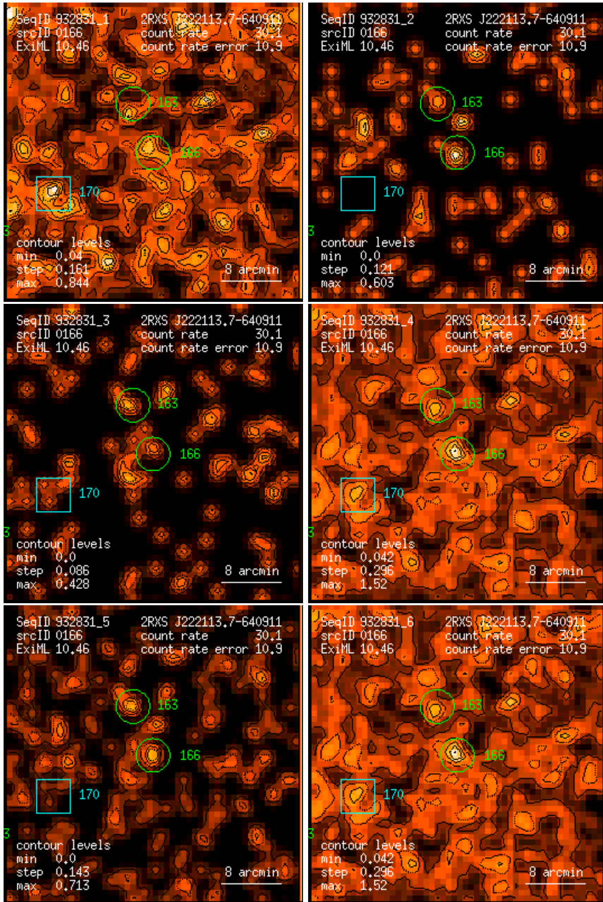
Figure 166: RASS 932831: detection 0166: band rate images, Gaussian filter: (1) PSPC channels 11 – 41, (2) 52 – 90, (3) 91 – 201, (4) 11 – 235, (5) 52 – 201, (6) 11 – 201. Broad band rates in counts/ks. Band rate contour levels in counts/ks/arcmin 2 .
