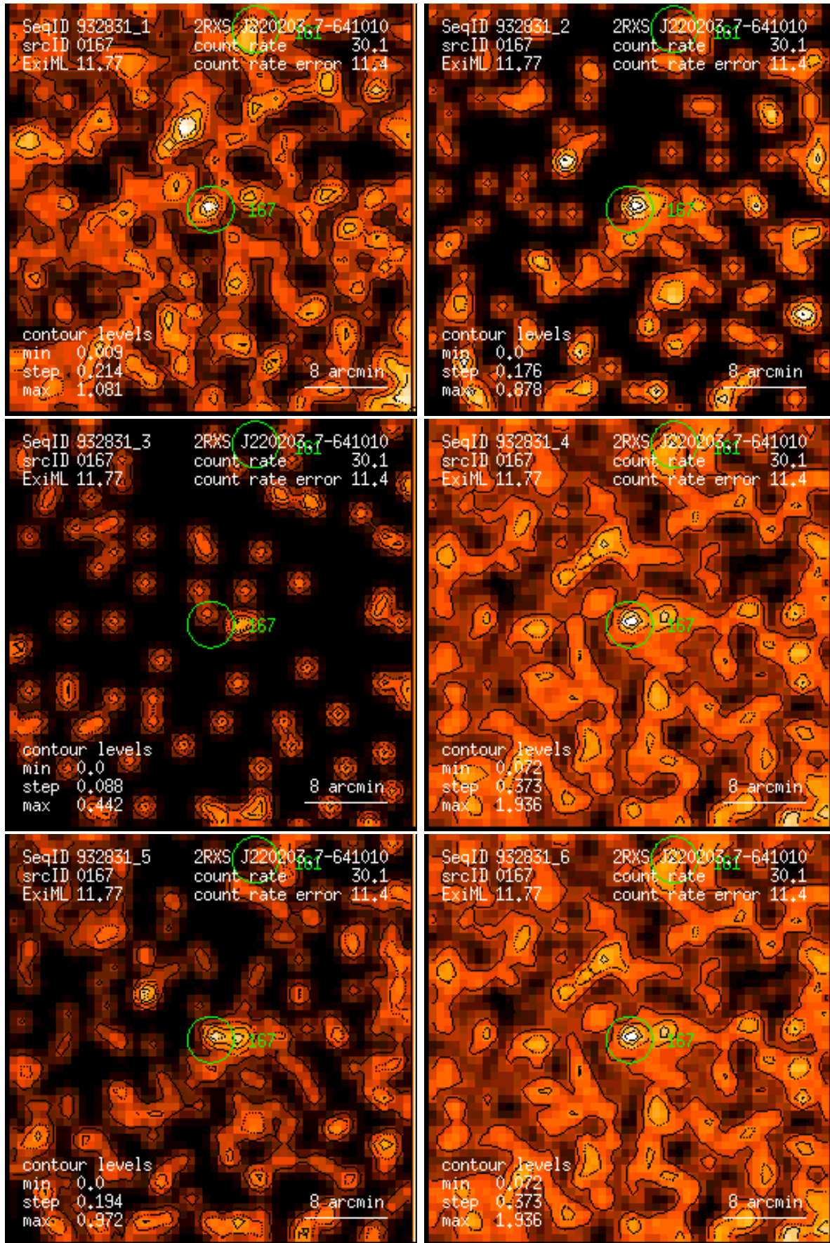
Figure 167: RASS 932831: detection 0167: band rate images, Gaussian filter: (1) PSPC channels 11 – 41, (2) 52 – 90, (3) 91 – 201, (4) 11 – 235, (5) 52 – 201, (6) 11 – 201. Broad band rates in counts/ks. Band rate contour levels in counts/ks/arcmin 2 .
