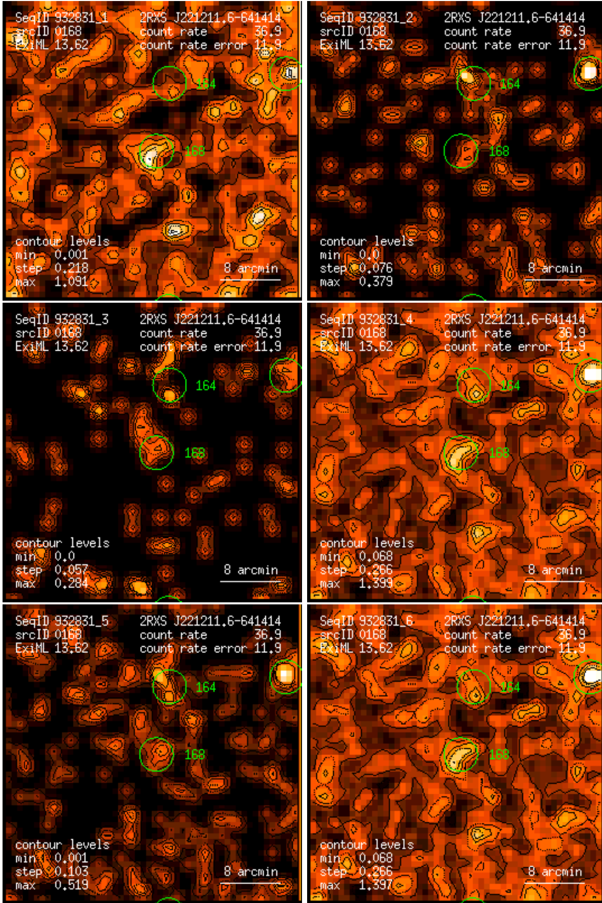
Figure 168: RASS 932831: detection 0168: band rate images, Gaussian filter: (1) PSPC channels 11 – 41, (2) 52 – 90, (3) 91 – 201, (4) 11 – 235, (5) 52 – 201, (6) 11 – 201. Broad band rates in counts/ks. Band rate contour levels in counts/ks/arcmin 2 .
