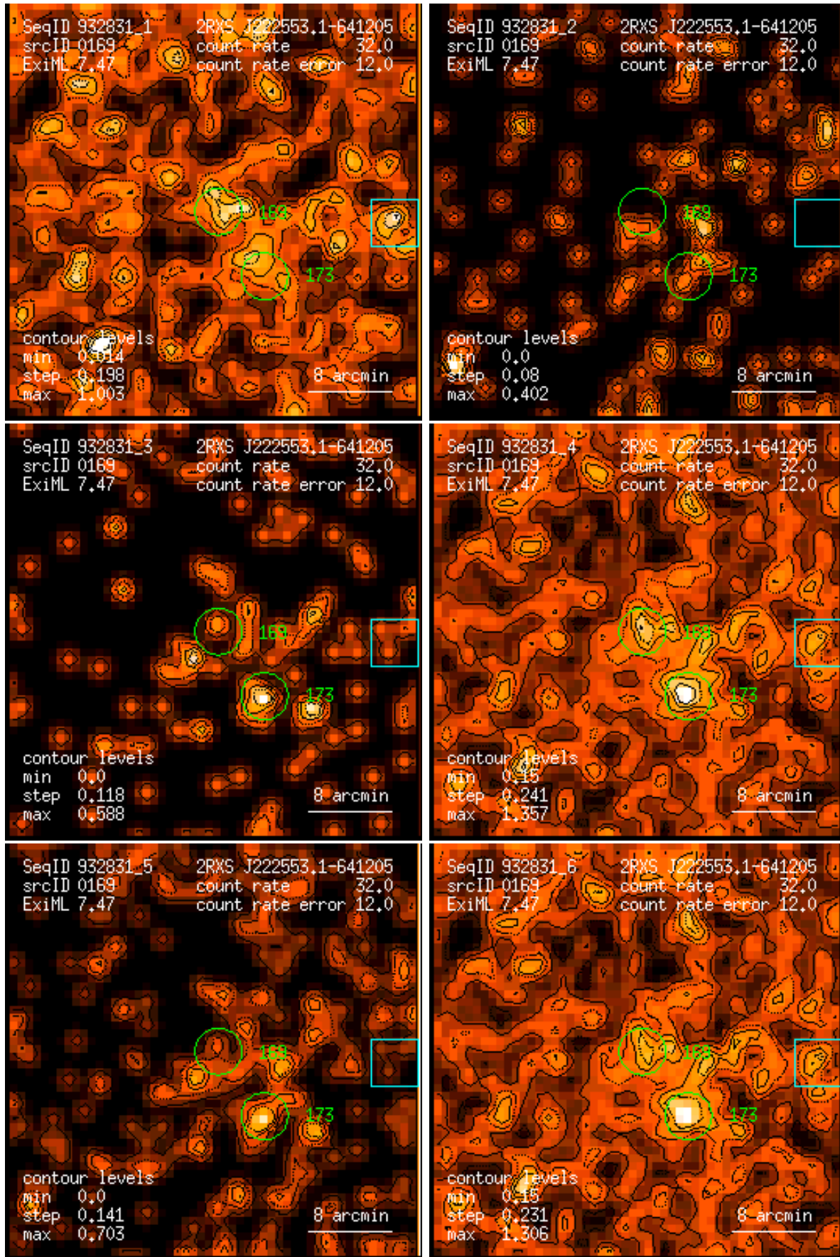
Figure 169: RASS 932831: detection 0169: band rate images, Gaussian filter: (1) PSPC channels 11 – 41, (2) 52 – 90, (3) 91 – 201, (4) 11 – 235, (5) 52 – 201, (6) 11 – 201. Broad band rates in counts/ks. Band rate contour levels in counts/ks/arcmin 2 .
