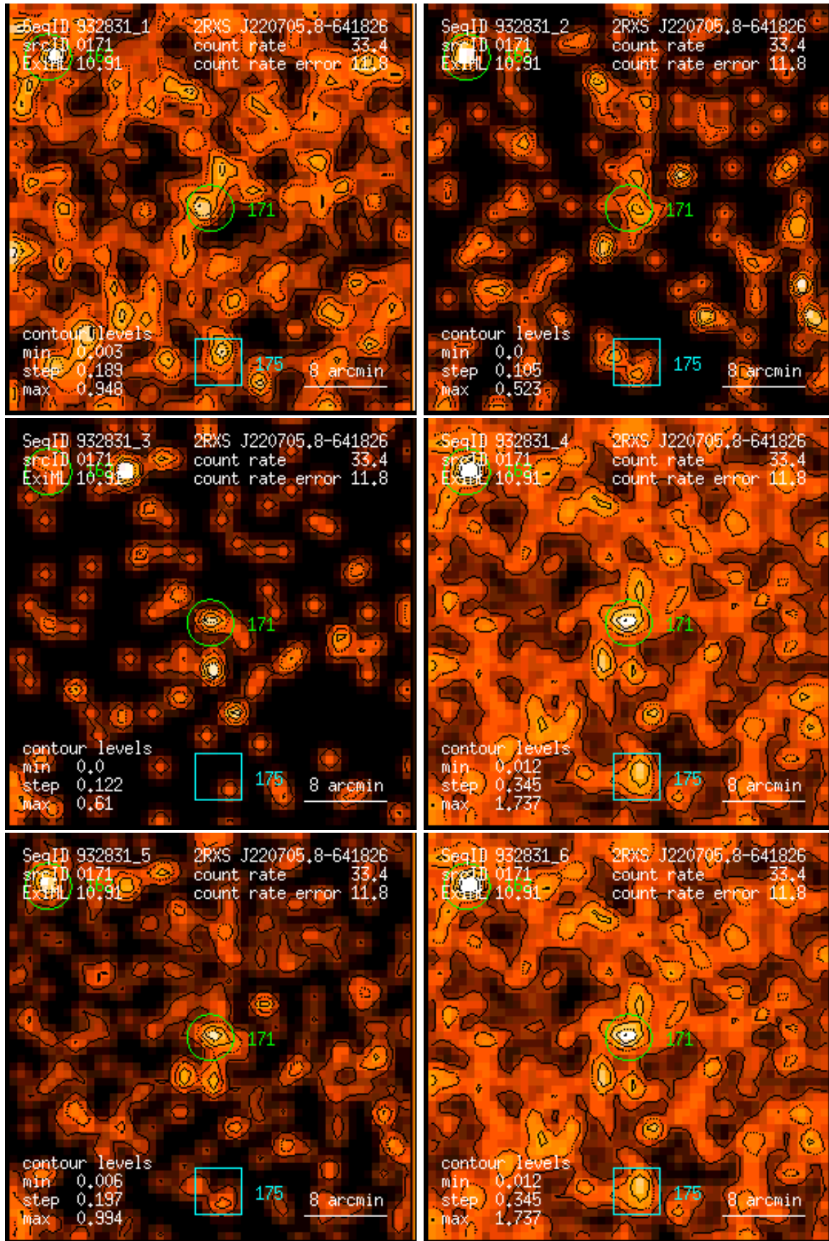
Figure 171: RASS 932831: detection 0171: band rate images, Gaussian filter: (1) PSPC channels 11 – 41, (2) 52 – 90, (3) 91 – 201, (4) 11 – 235, (5) 52 – 201, (6) 11 – 201. Broad band rates in counts/ks. Band rate contour levels in counts/ks/arcmin 2 .
